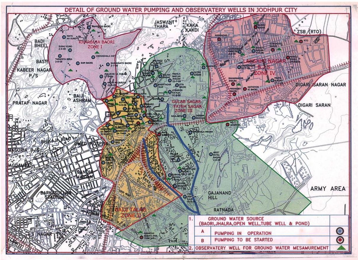
Fig.1: Map showing zones affected with rising water level problem of Jodhpur city.
