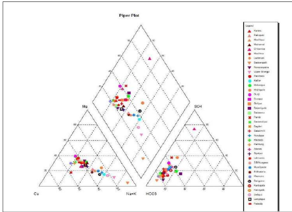
Fig.16a. Piper diagram for deeper aquifer, Koraput District
