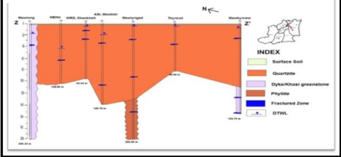
Fig. 3.8 Section along Mawiong-Mawkynrew
