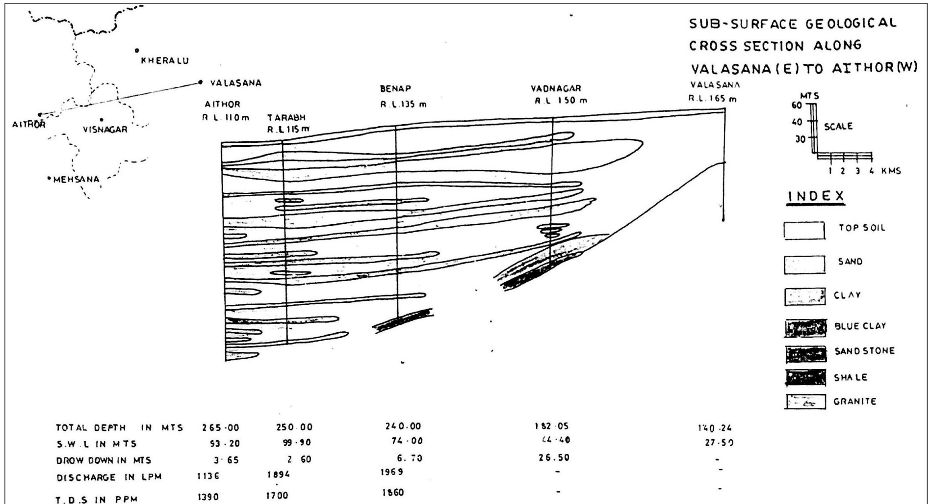
Figure – 20 Hydrogeological cross section along Valasana(Kharalu Taluk) to Arthor (Unjha Taluka) of Mahesana-Patan District
