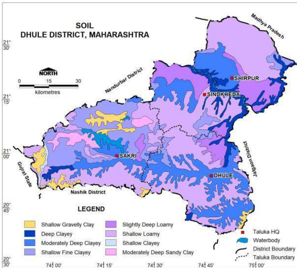
Figure 1.6: Soil, Dhule District
