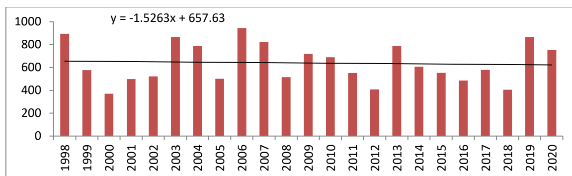
Figure 1.7: Rainfall Analysis (1998-2020), Dhule District
