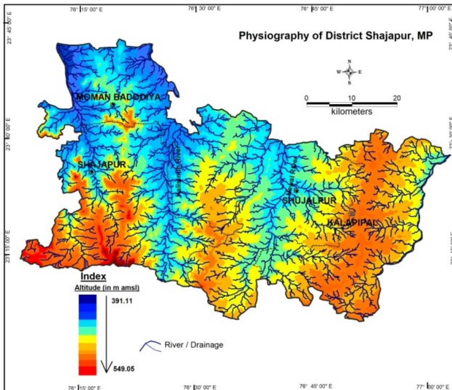
Figure No.6 Physiographic Map of Shajapur district
