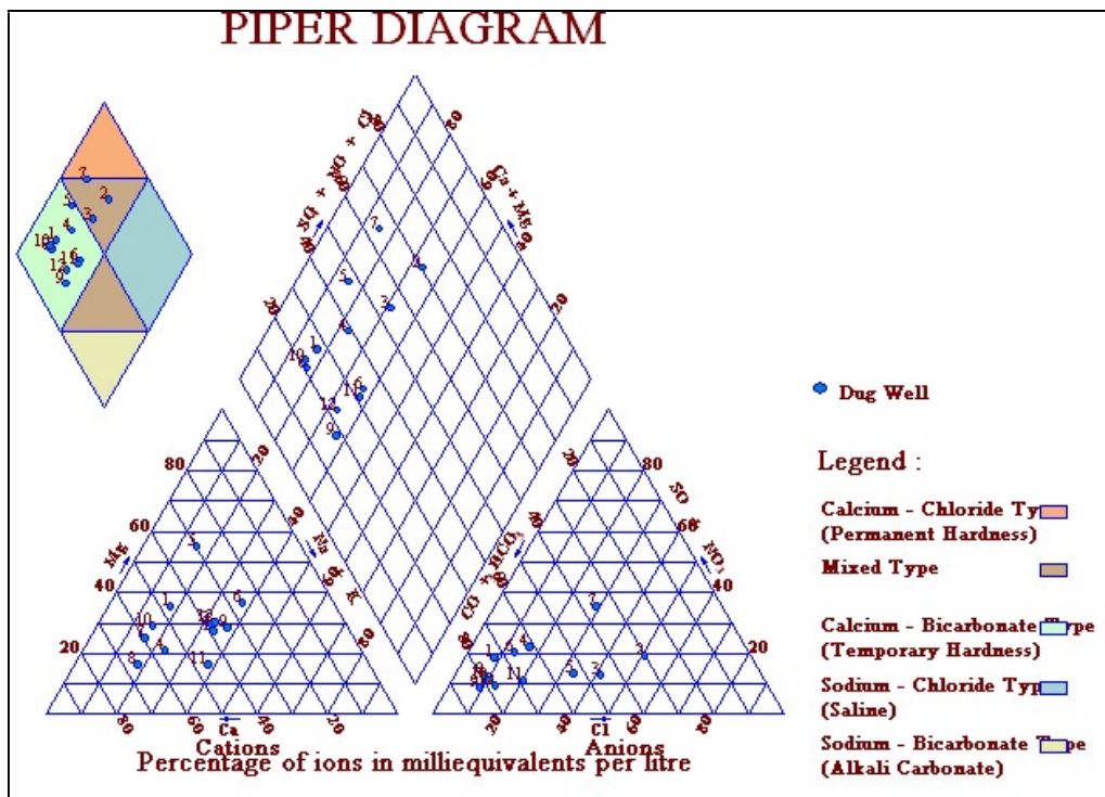
Figure No.20: Piper Diagram showing distribution of cations and anions
