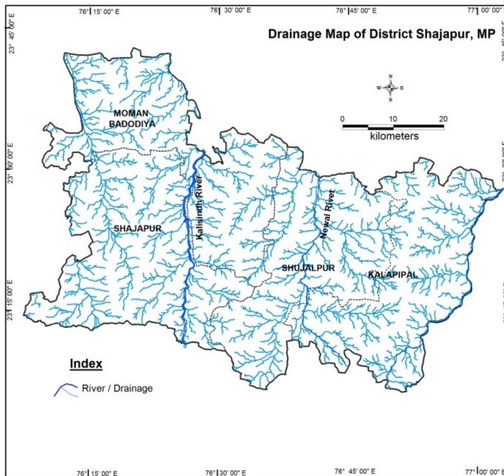
Figure No.7: Drainage Map of Shajapur district
