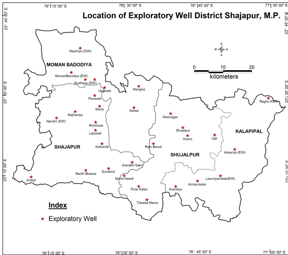
Figure No.15: Map showing location of exploratory wells in Shajapur district
