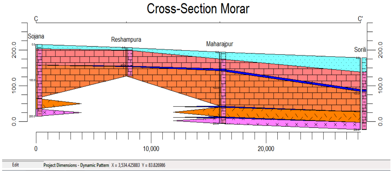
Fig 21: Artificial Recharge Structures location Map and 2D section of Morar Block
