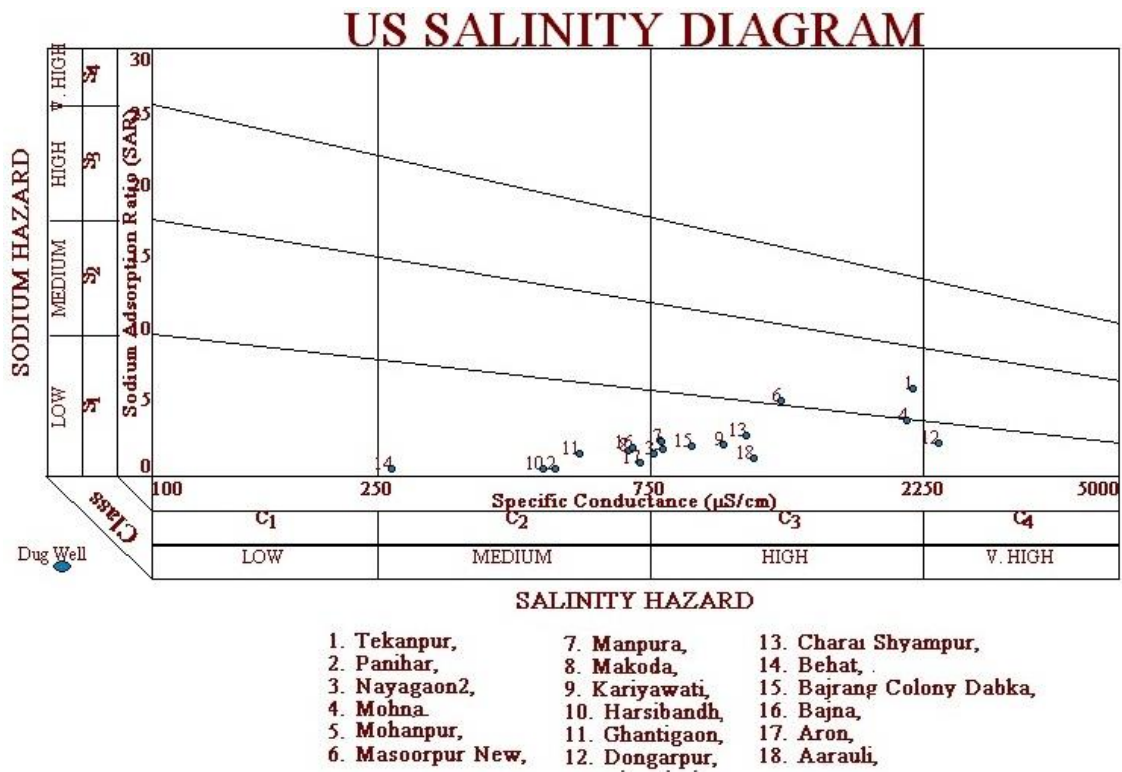
Fig. 16 US Salinity Diagram for water samples collected from National Hydrograph Stations of Gwalior District, Madhya Pradesh
