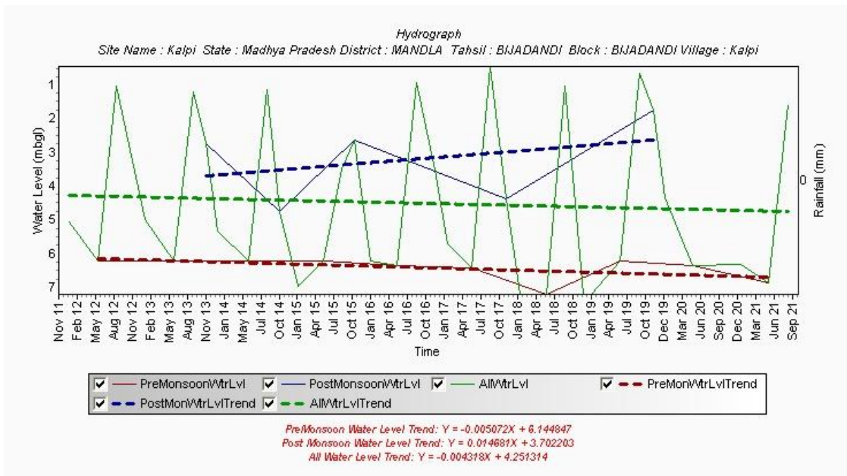
Fig. No. 18: Hydrograph of Kalpi dug well, Bijadandi Block
