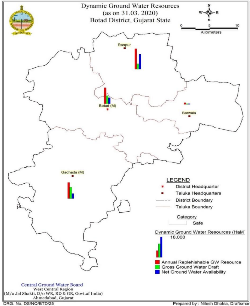
Figure 34: Dynamic Groundwater Resources Botad District.
