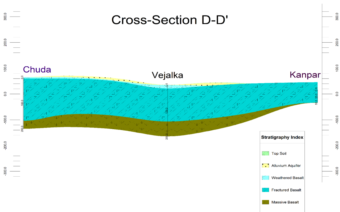
Figure 17: Hydrogeological cross section between Chuda and Kanpar.
