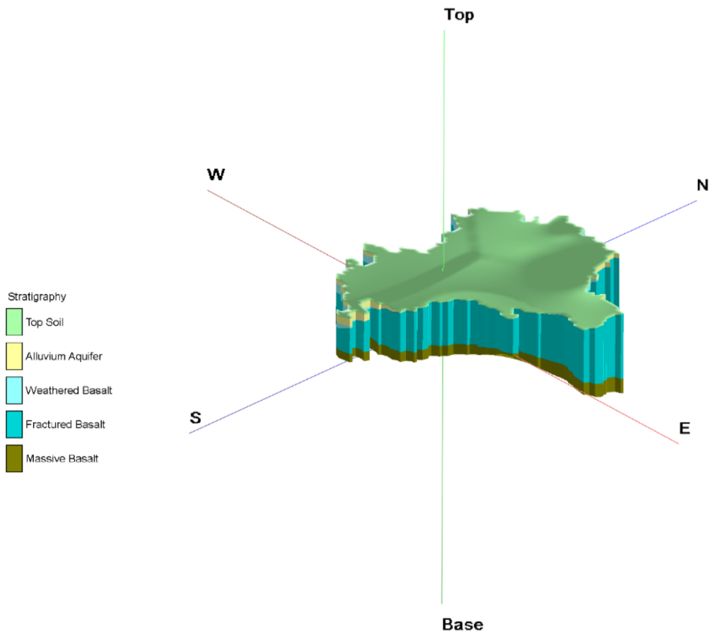
Figure 18: 3D Model/ Aquifer disposition of Botad District.
