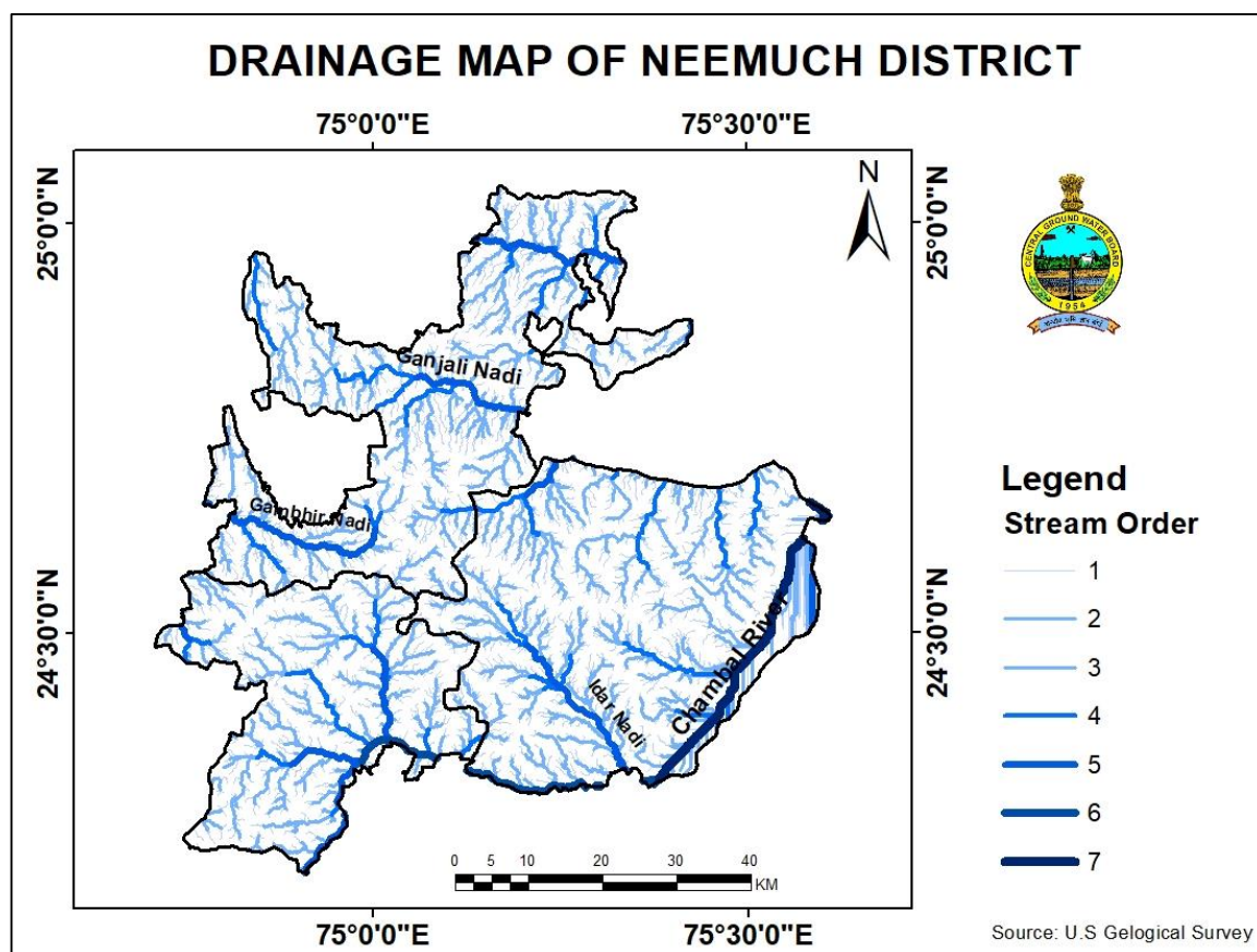
Fig.1.7: Drainage map
