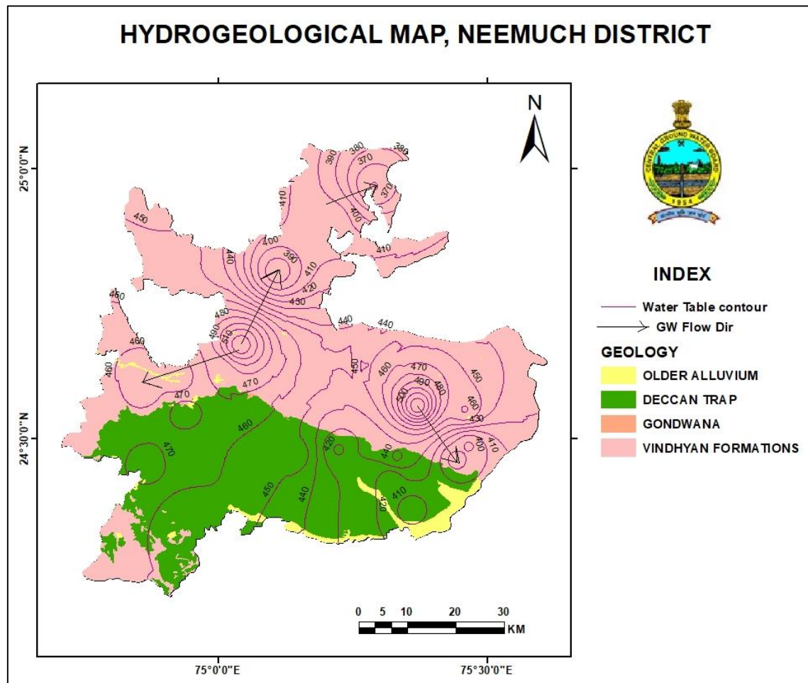
Fig.3.1:Hydrogeological Map.
