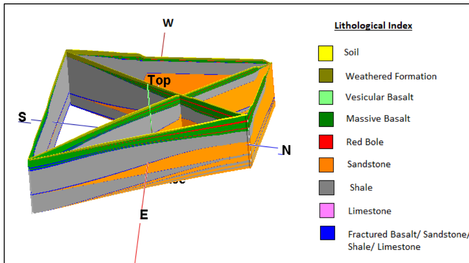
Fig.7.12: Fence Diagram, Neemuch block
