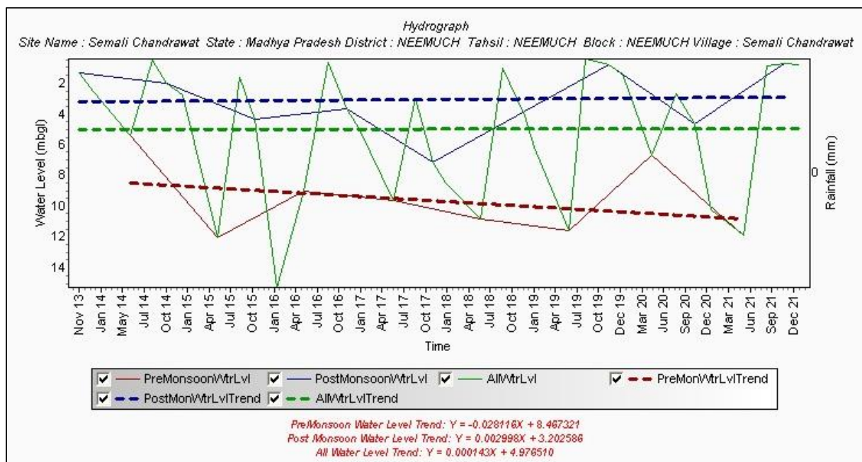
Fig.7.15: Hydrograph, Village-Semali Chandrawat, Block- Neemuch
