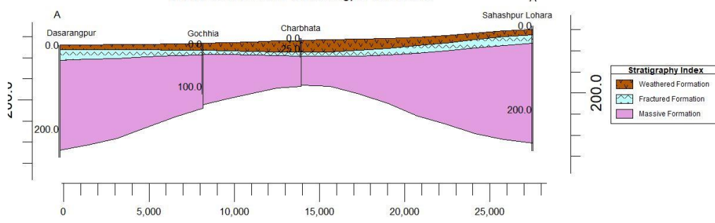
Figure 19: Two Dimensional (2-D) Aquifer Disposition of Kabirdham district
