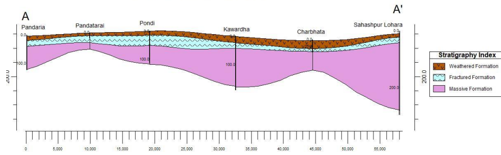
Cross-Section from Pandariya to Lohara
