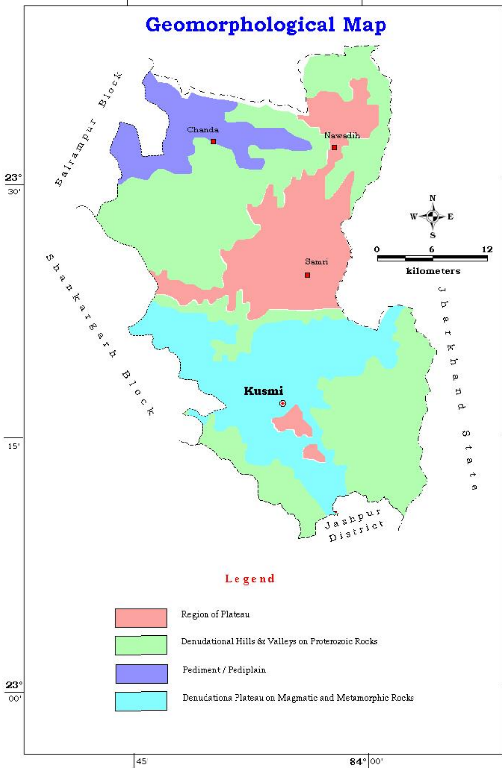
Figure 2 Geomorphology Map of Kusmi Block
