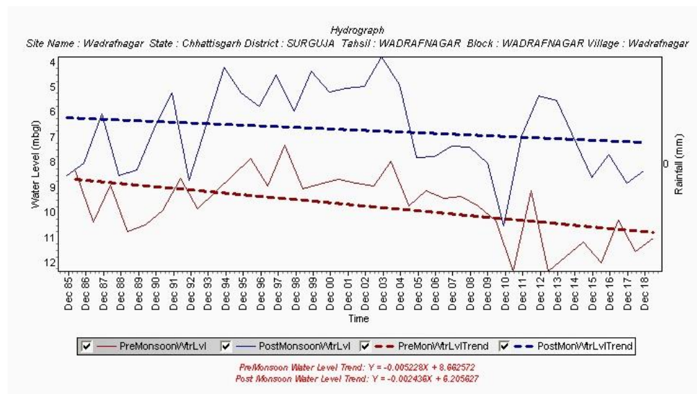
Figure 10 b: Hydrograph of Wadrafnagar town, Wadrafnagar block
