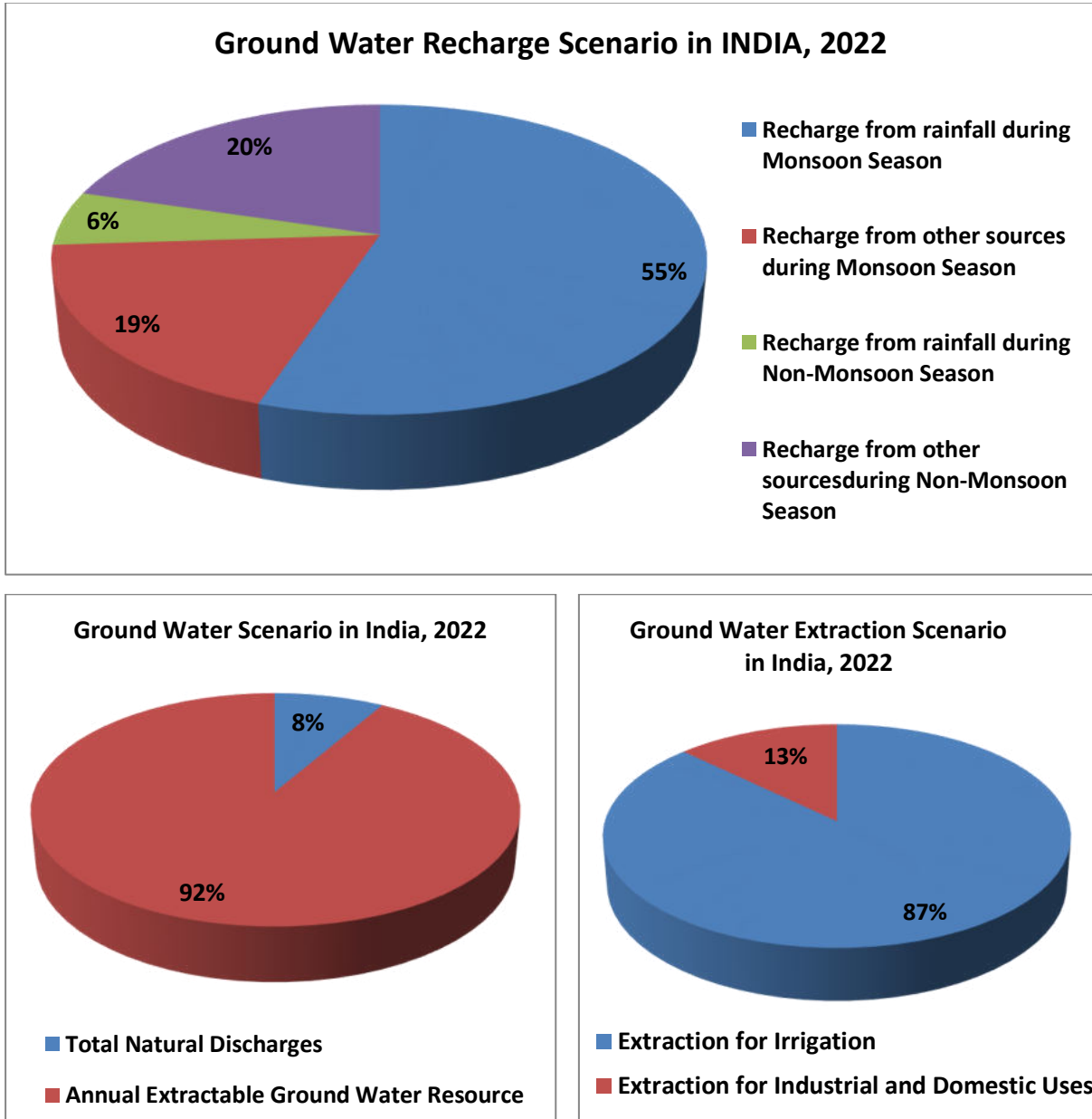
Fig-6.1: Ground Water Resources and Extraction Scenario in India, 2022
