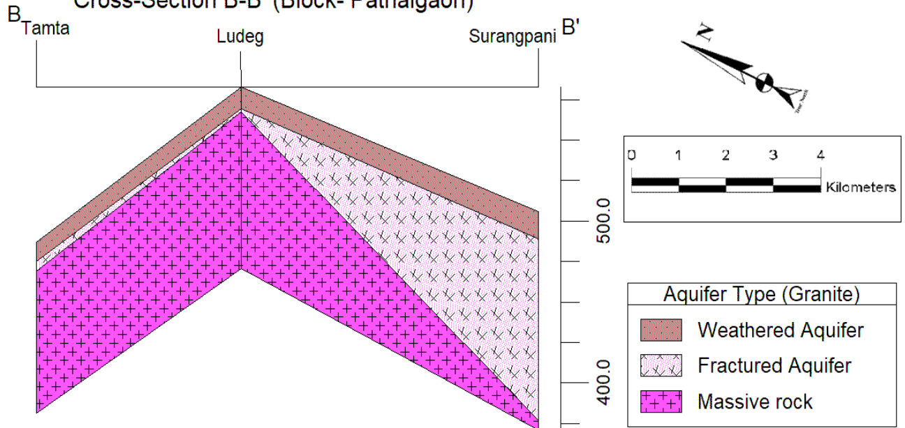
Figure 14 2D Cross-Section of Pathalgaon block
