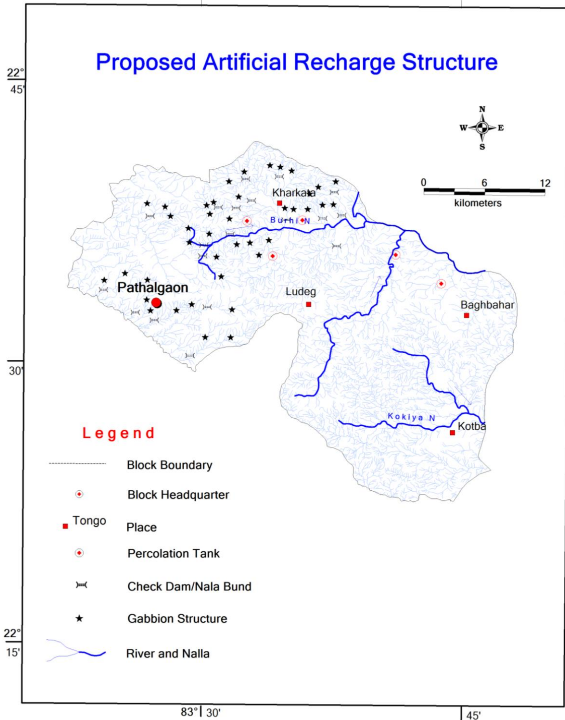
Figure 16 Location of proposed Artificial Recharge Structure
