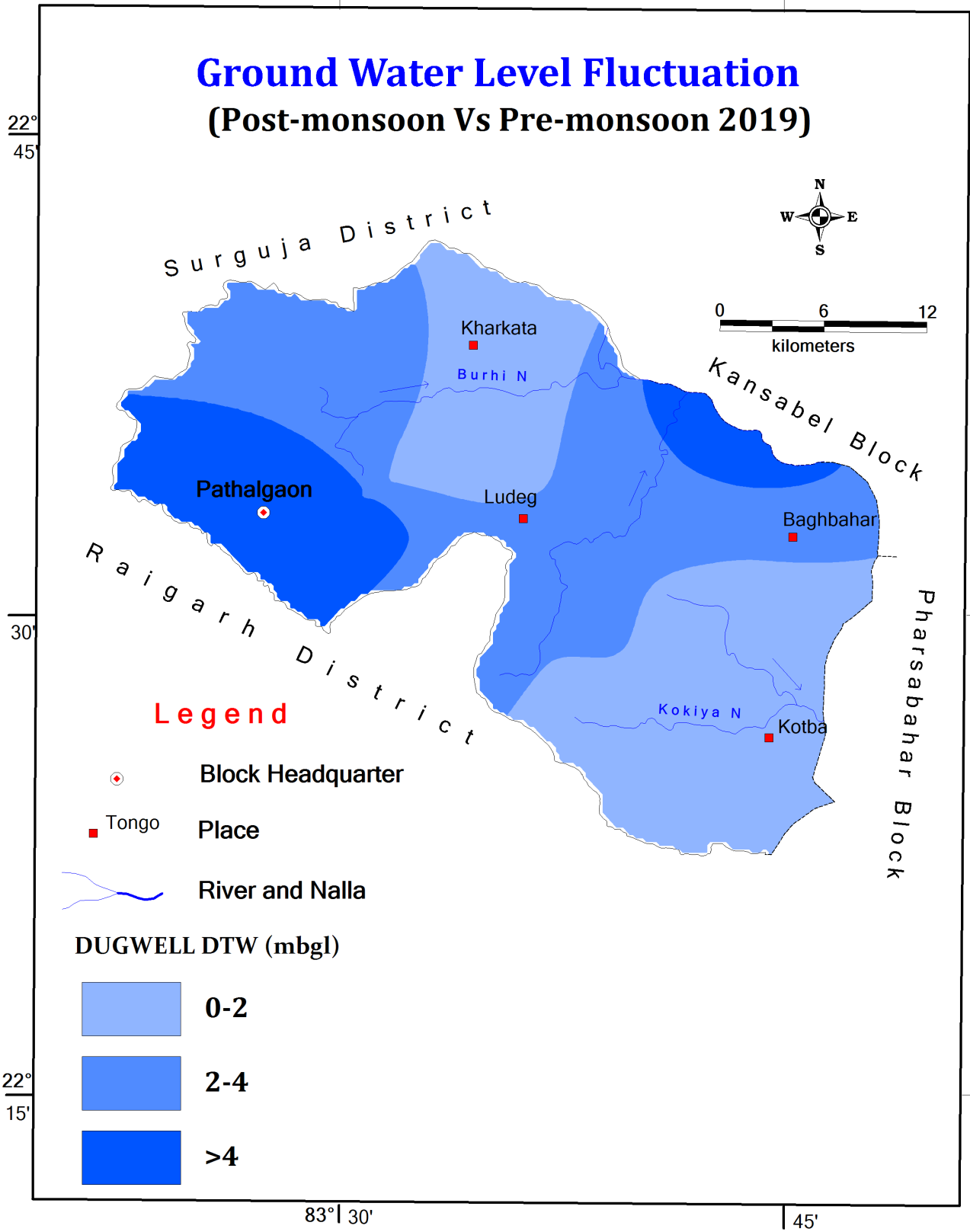
Figure 6 Seasonal waterlevel fluctuation of Phreatic Aquifer
