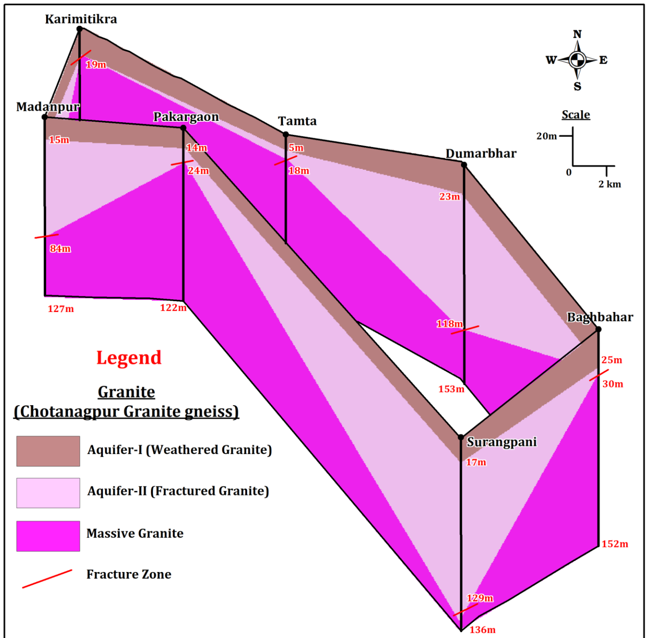
Figure 15 Fence diagram of Pathalgaon block
