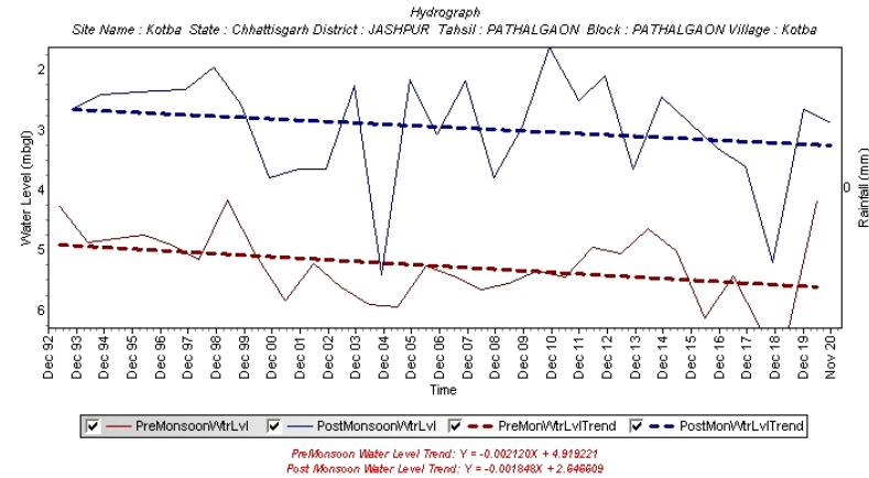
Figure 11 Hydrograph of Kotba village, Pathalgaon block
