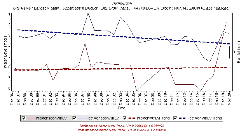
Figure 10 Hydrograph of Bangaon village, Pathalgaon block
