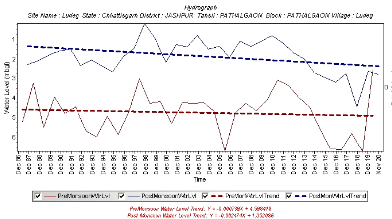
Figure 12 Hydrograph of Ludeg village, Pathalgaon block
