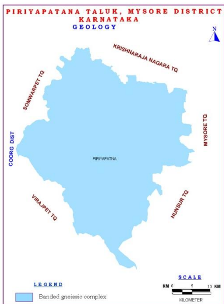
Fig-6: Geology Map
