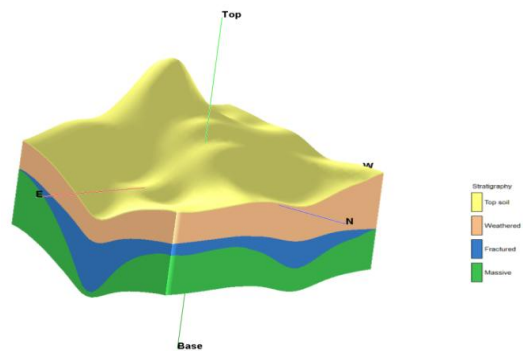
Fig-13d
