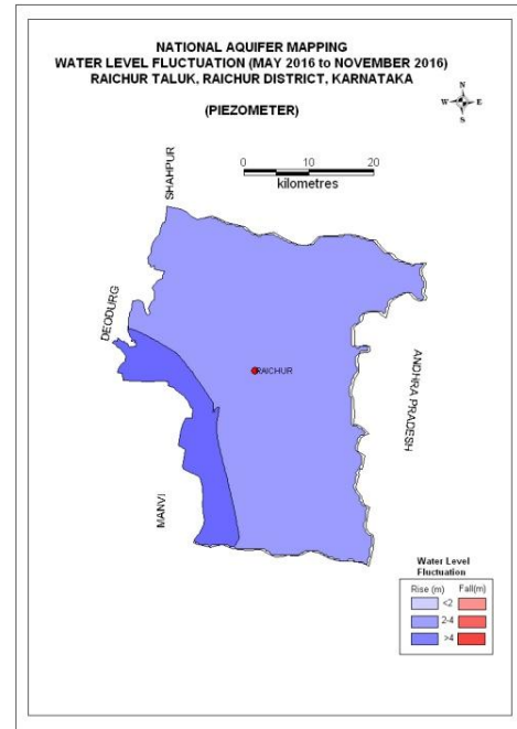
Fig 11: Seasonal water level fluctuation (Aq- II)
