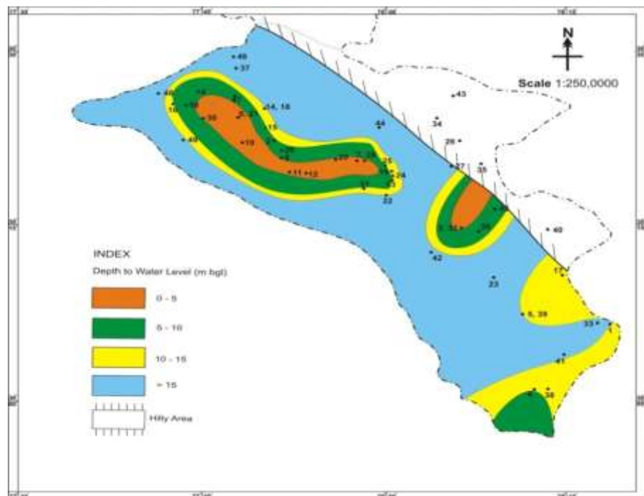
Fig. 10 Depth to Water Level, Dehradun, November, 2013
