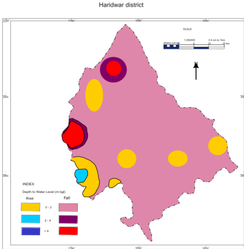
Figure 17 Annual Water Level Fluctuation Map (May 2015 vs 2016), Haridwar District
