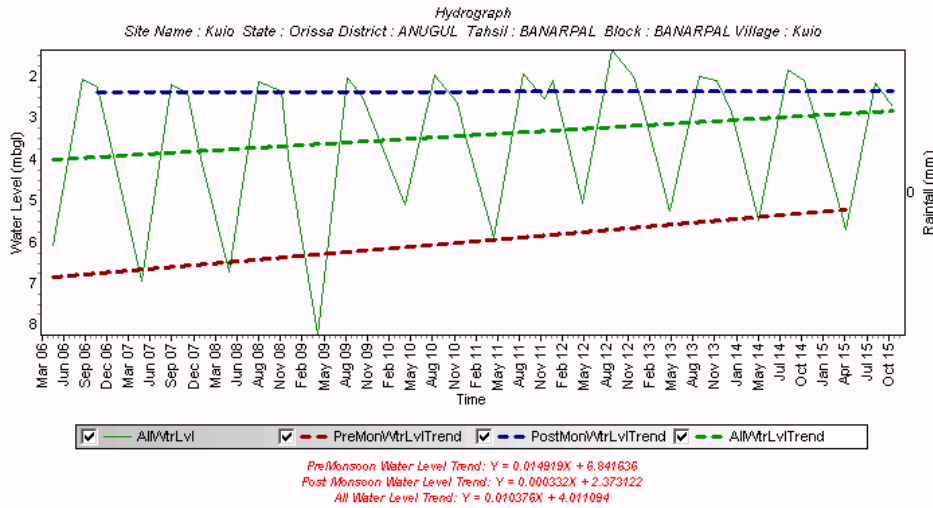
Fig. 4.9d: Hydrograph (2006-15), Kuio, Banarpal block, Angul district
