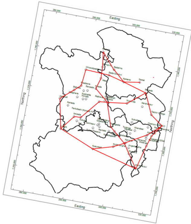
Fig. 6.4: 3-D Fence diagram, NAQUIM area, Angul district
