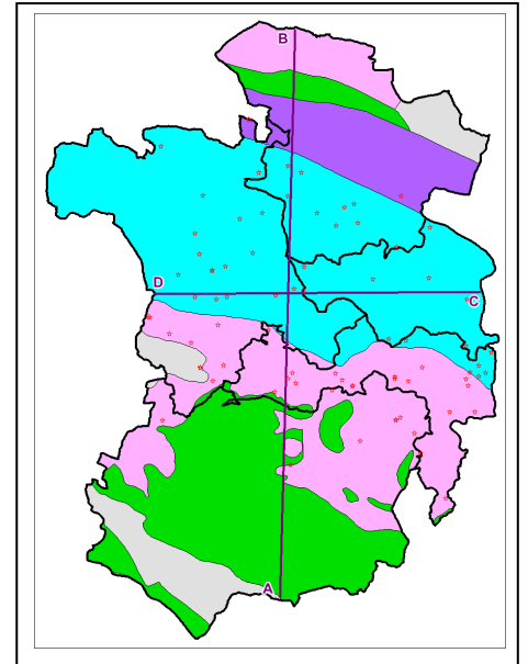
Fig. 6.2b: Delineation of Aquifers I & II from Lithological Section in the NAQUIM area, Angul district.
