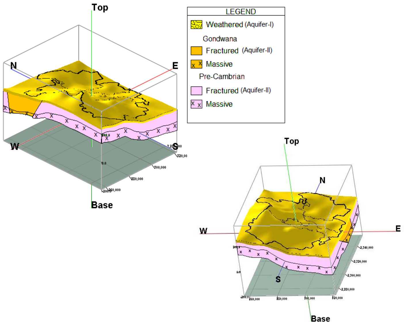
Fig. 6.3: Schematic 3-D Aquifer Disposition in NAQUIM area, Angui aistrict
