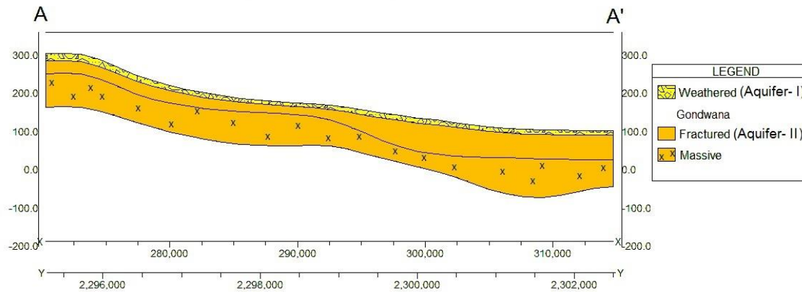
Cross-Section A-A'
