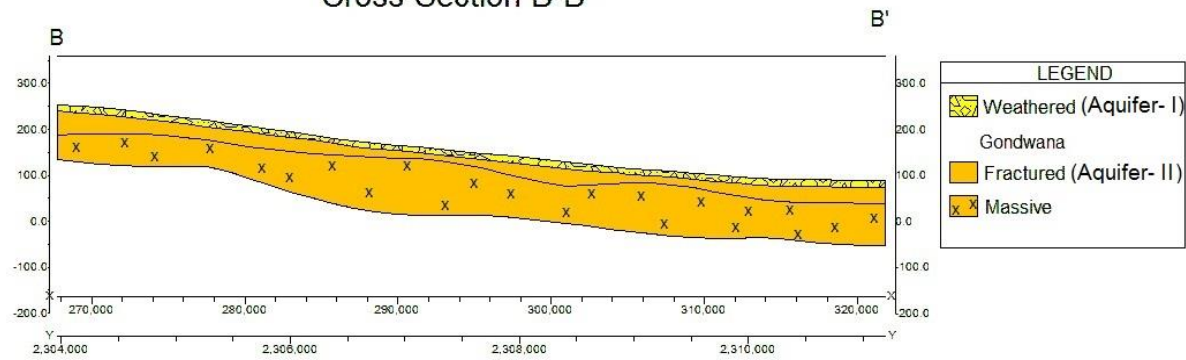
Cross-Section B-B'
