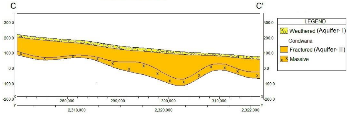
Cross-Section C-C'
