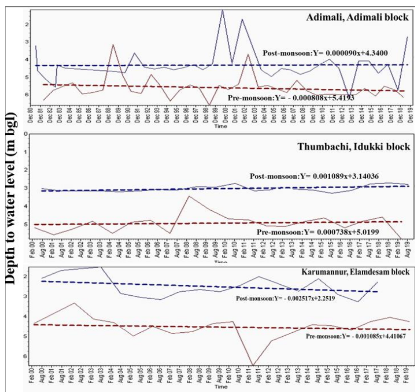
Figure 3.11. Hydrographs of selected GWMWs in Idukki district.
