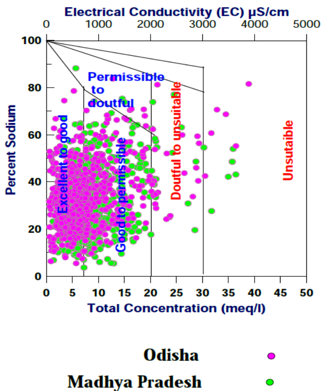
Figure 48: Plots of sodium percent verses electrical conductivity (after Wilcox 1955) in groundwater samples in Odisha and Madhya Pradesh.
