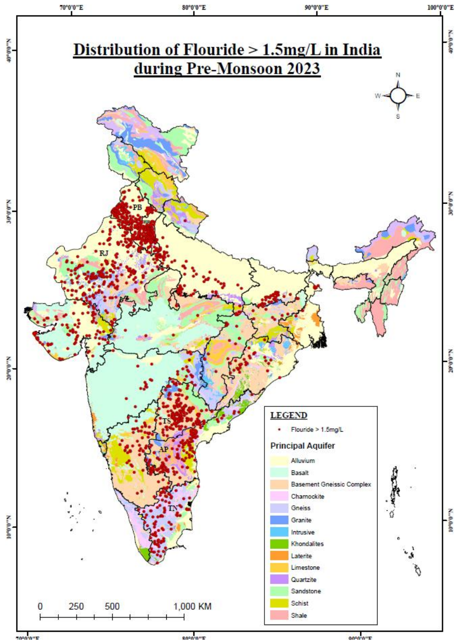
Figure 13: Locations having Fluoride concentration >1.5 mg/L during Pre-Monsoon 2023.
