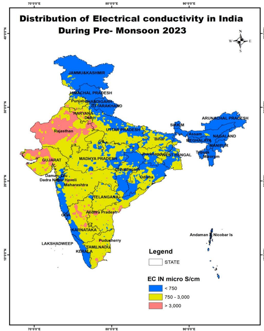
Figure 3: Distribution of Electrical Conductivity in India during Pre-monsoon (May, 2023).
