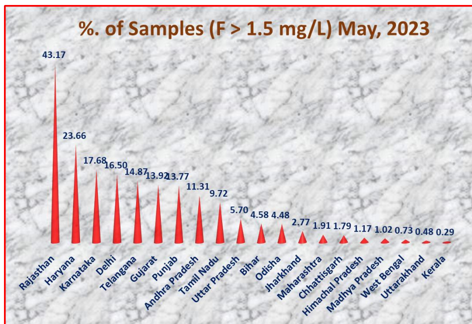
Figure 15: State-wise % of water samples with Fluoride concentration > 1.5 mg/L during pre-monsoon,2023.
