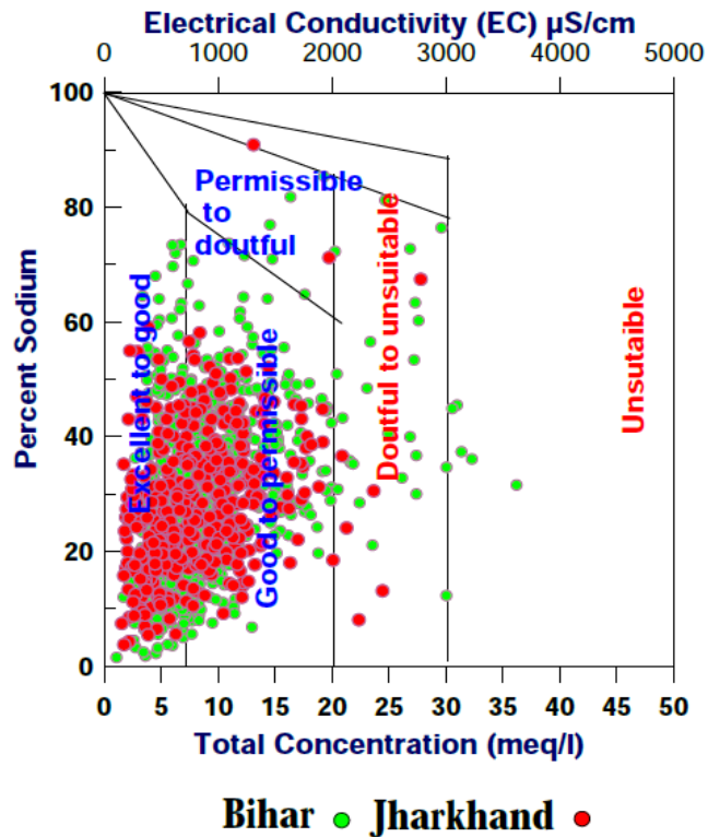
Figure 47: Plots of sodium percent verses electrical conductivity (after Wilcox 1955) in groundwater samples Bihar and Jharkhand.
