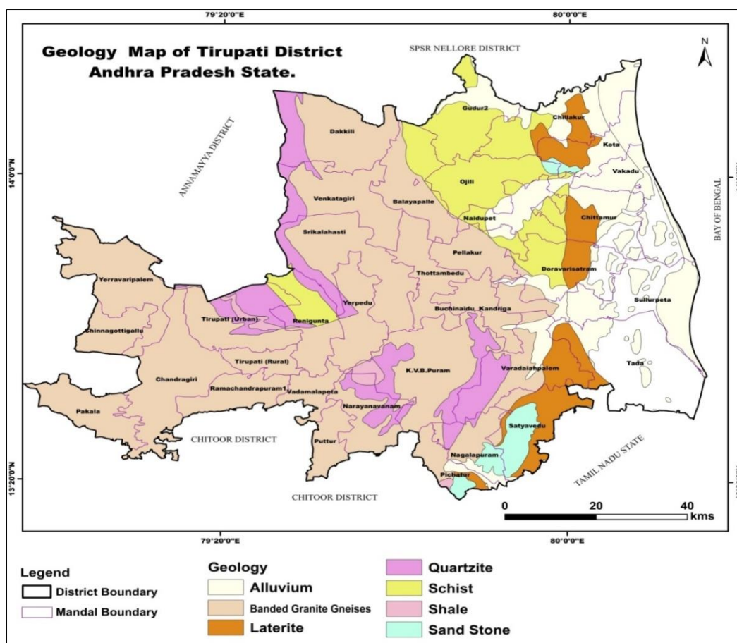
Figure 8 Geology of Tirupati district
