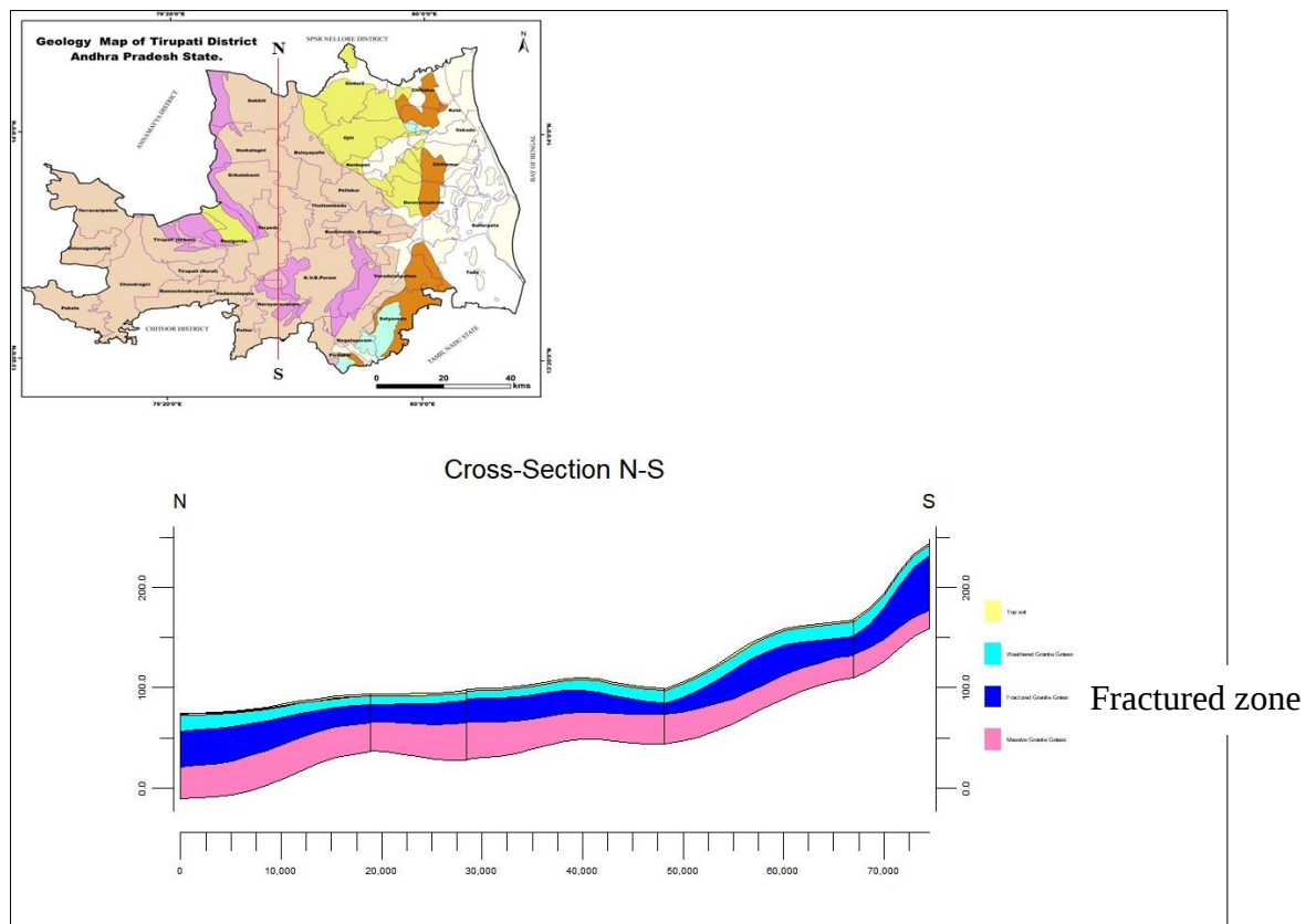
Figure 23.2 D model of N-S cross Section
