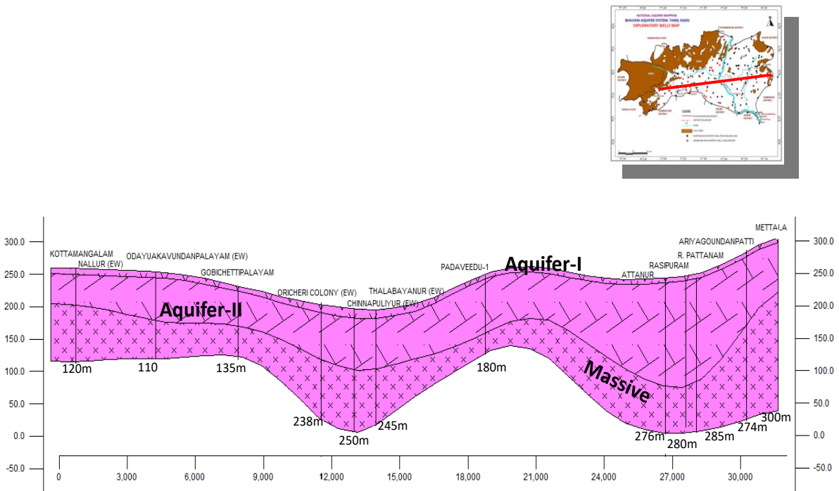
Fig-3.12 Hydrogeological cross section
