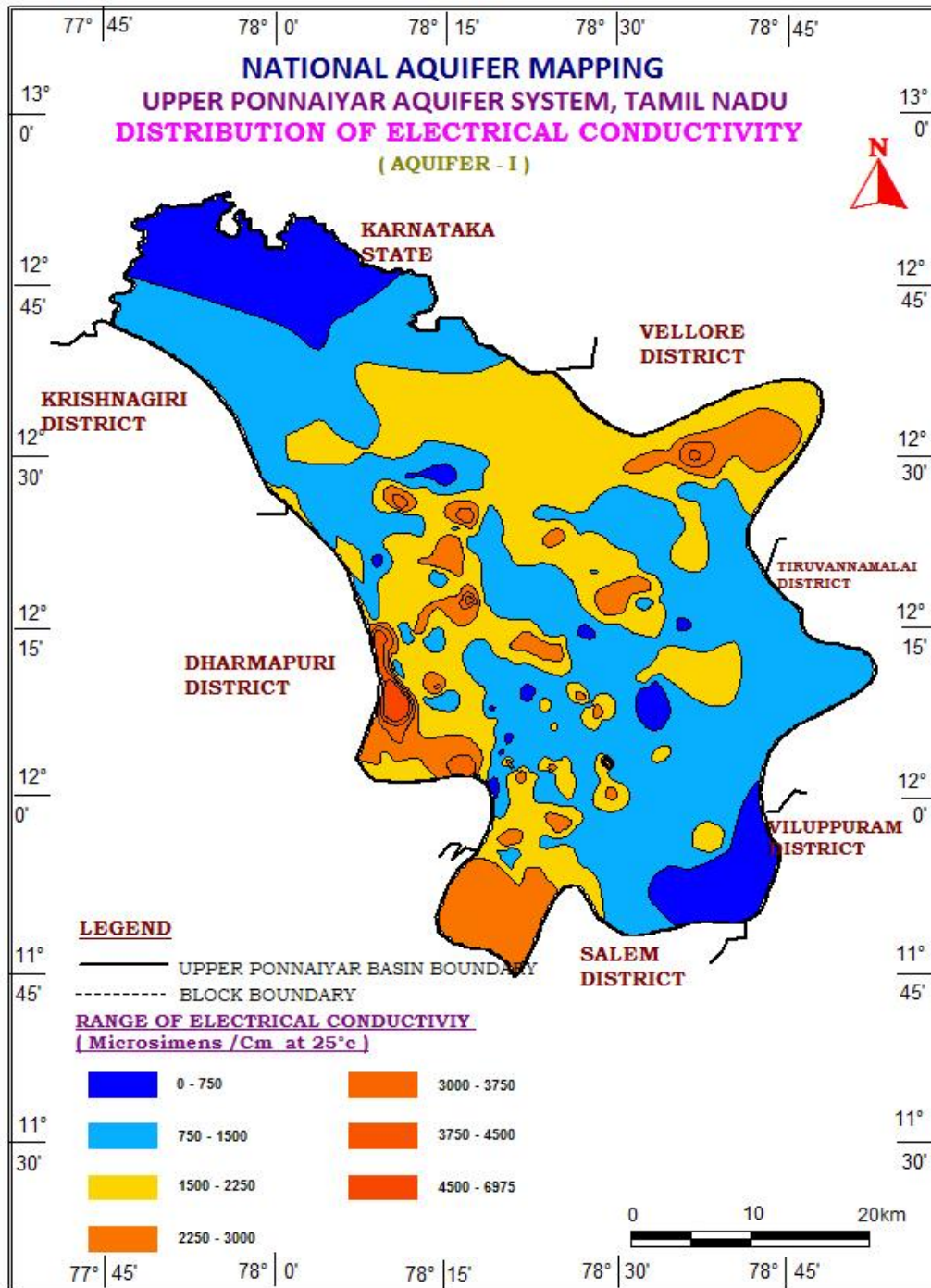
Figure 8.1 Distribution of Electrical Conductivity in shallow aquifer (Aquifer-I)
