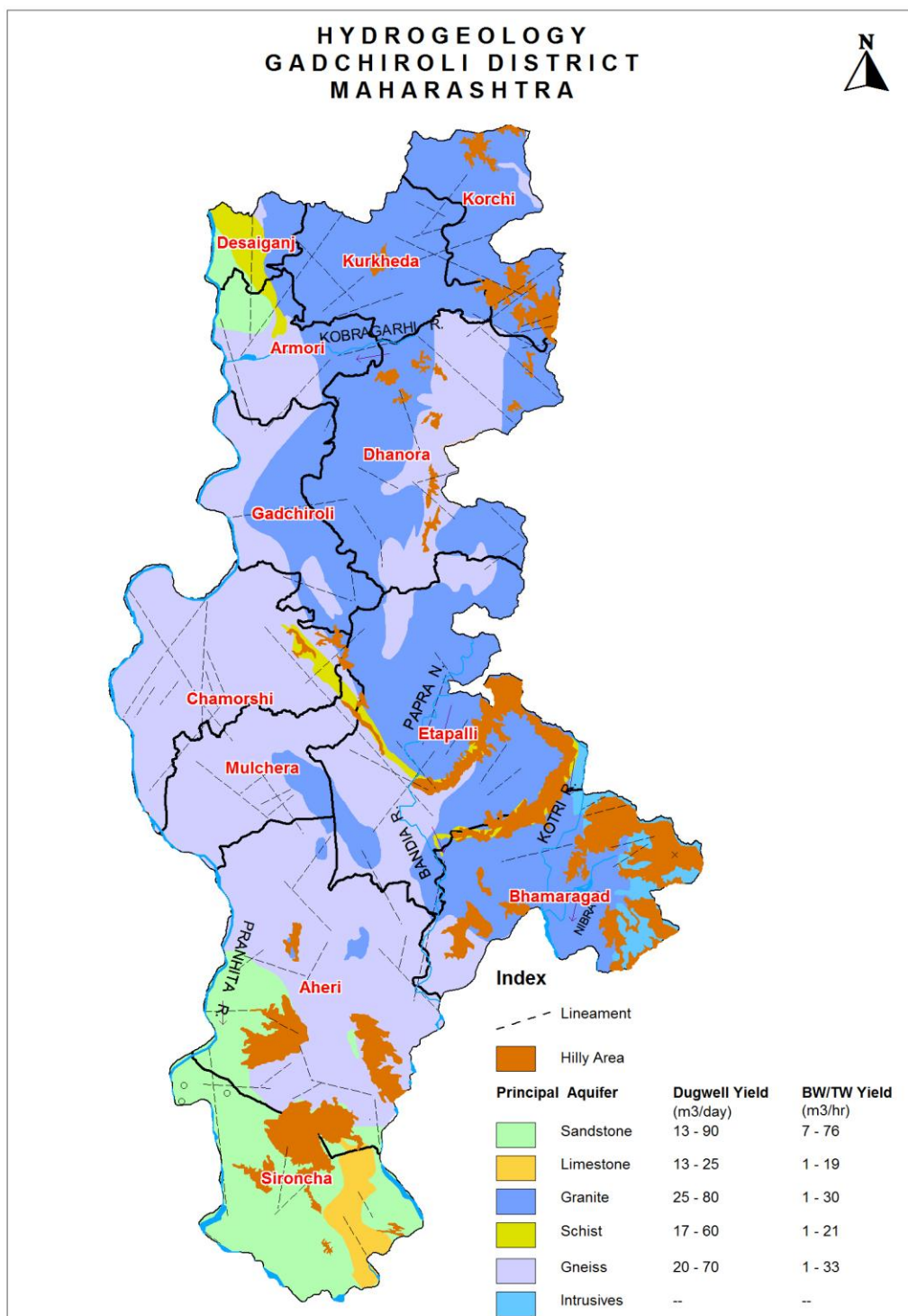
Figure-2: Hydrogeology
