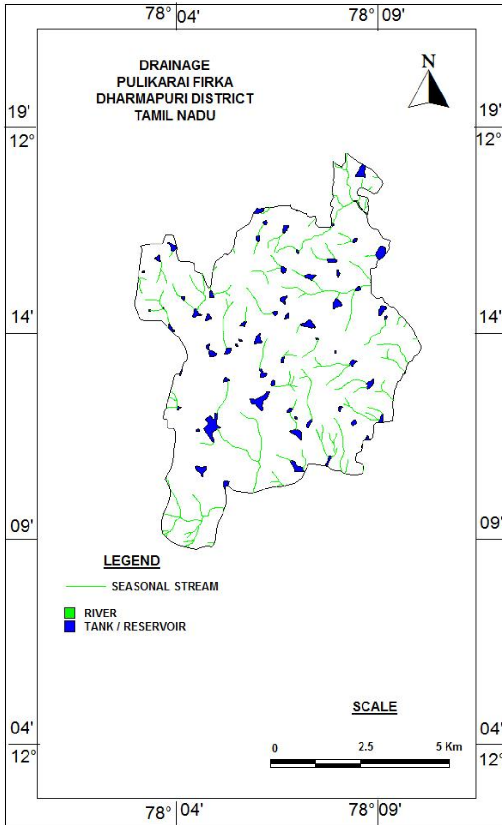
4.Drainage map of Pulikarai Firka
