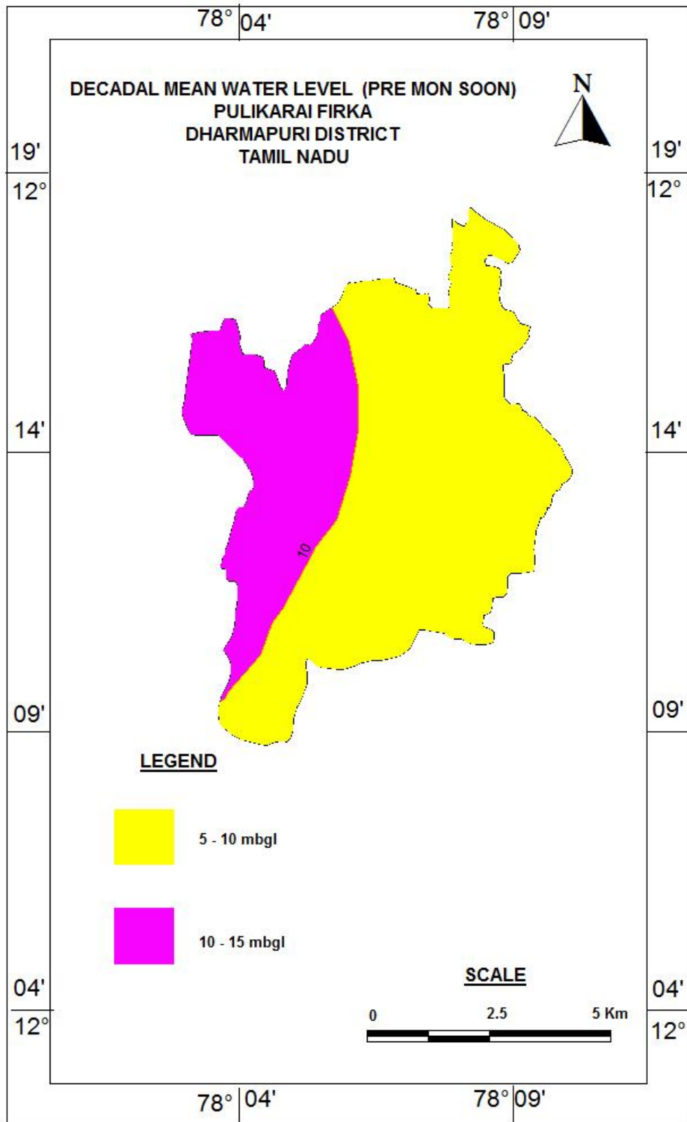
Figure 6a. Decadal Pre -monsoon water level in Pulikarai firka
