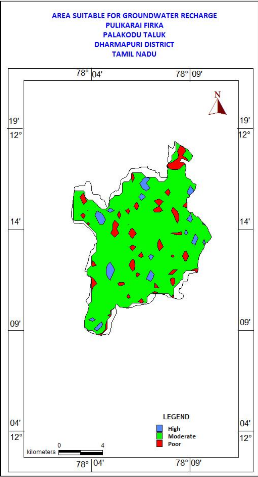
Figure .7 showing recharge worthy area
