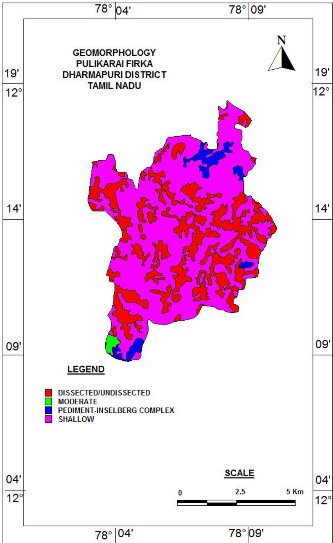
Figure 2. Geomorphology of Pulikarai Firka
