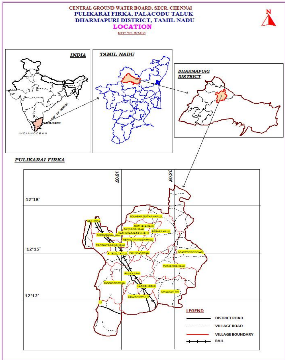
Figure 1. Location map of Pulikarai firka
