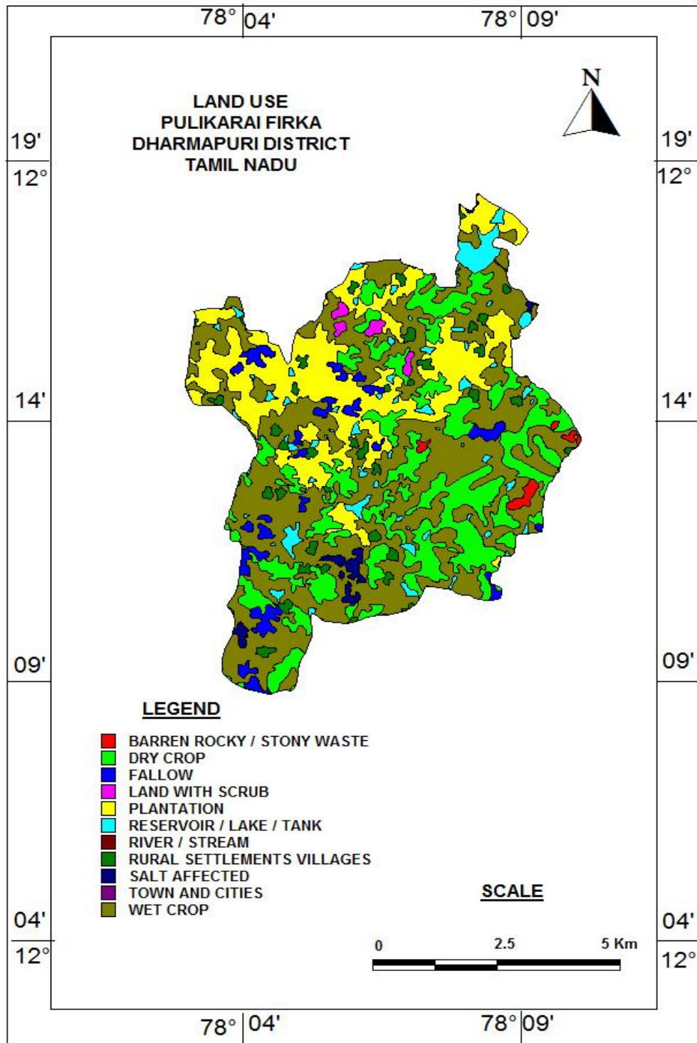
Figure 3. Landuse map of Pulikarai Firka
