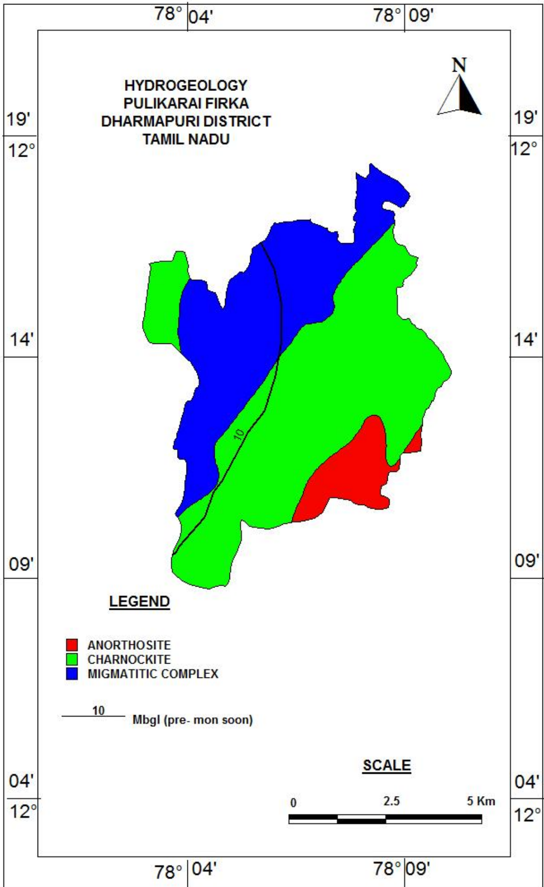
Figure 5. Hydrogeological Map of Pulikarai Firka
