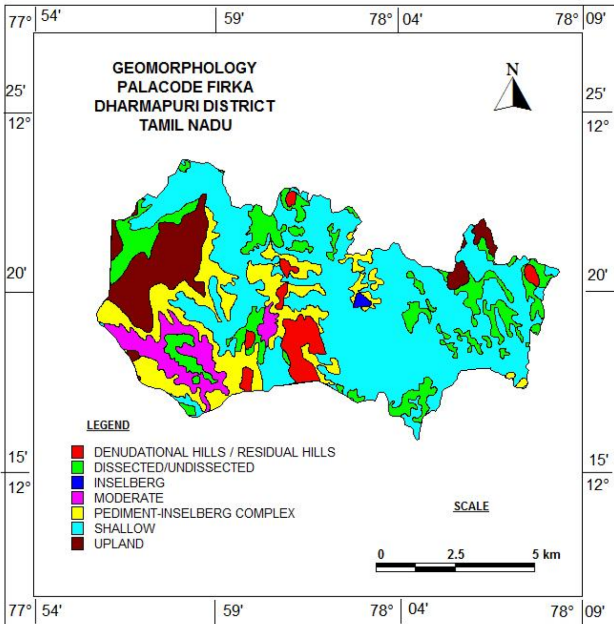
Figure 2. Geomorphology of Palacode Firka
