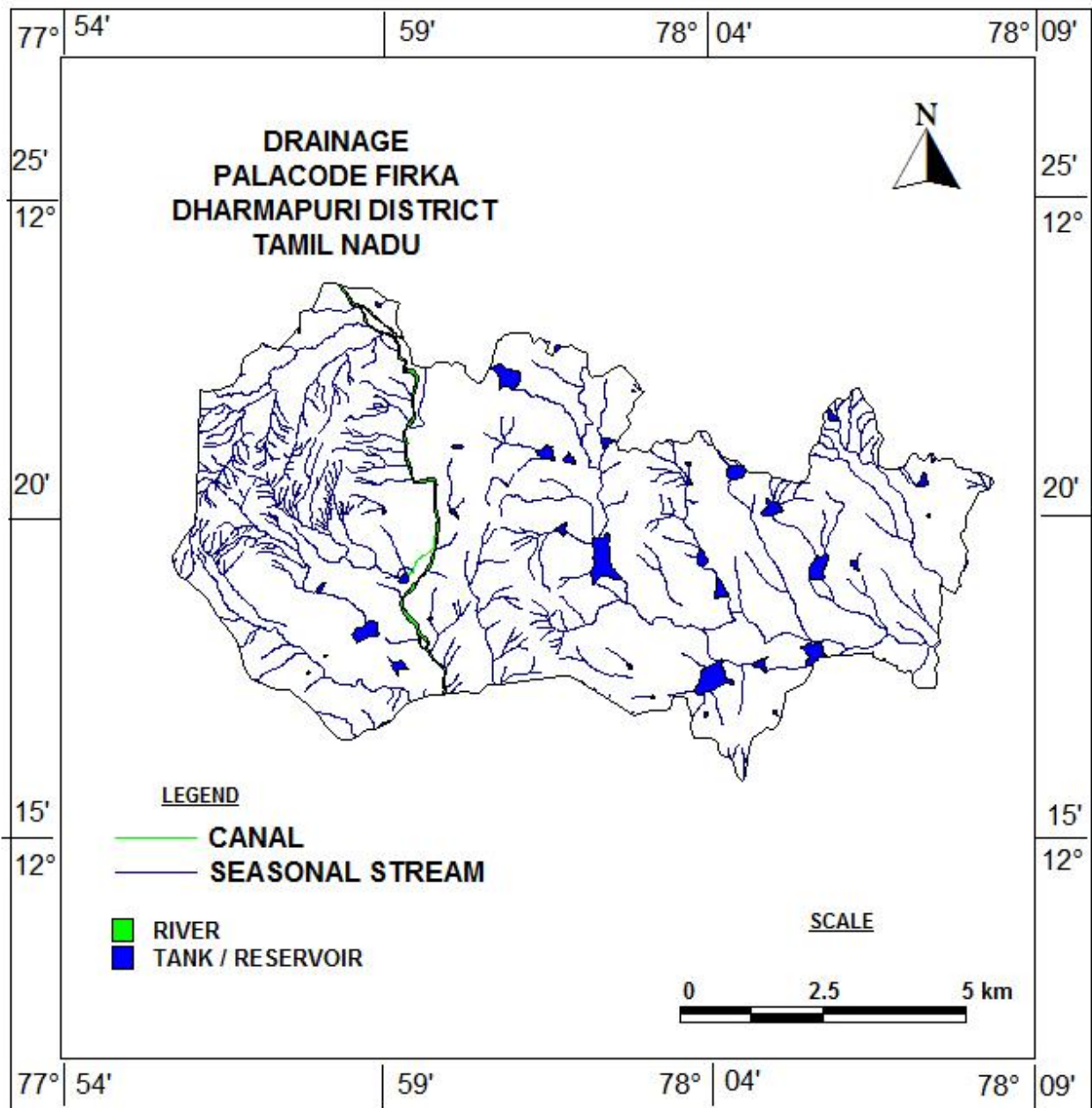
Figure 4. Drainage map of Palacode Firka
