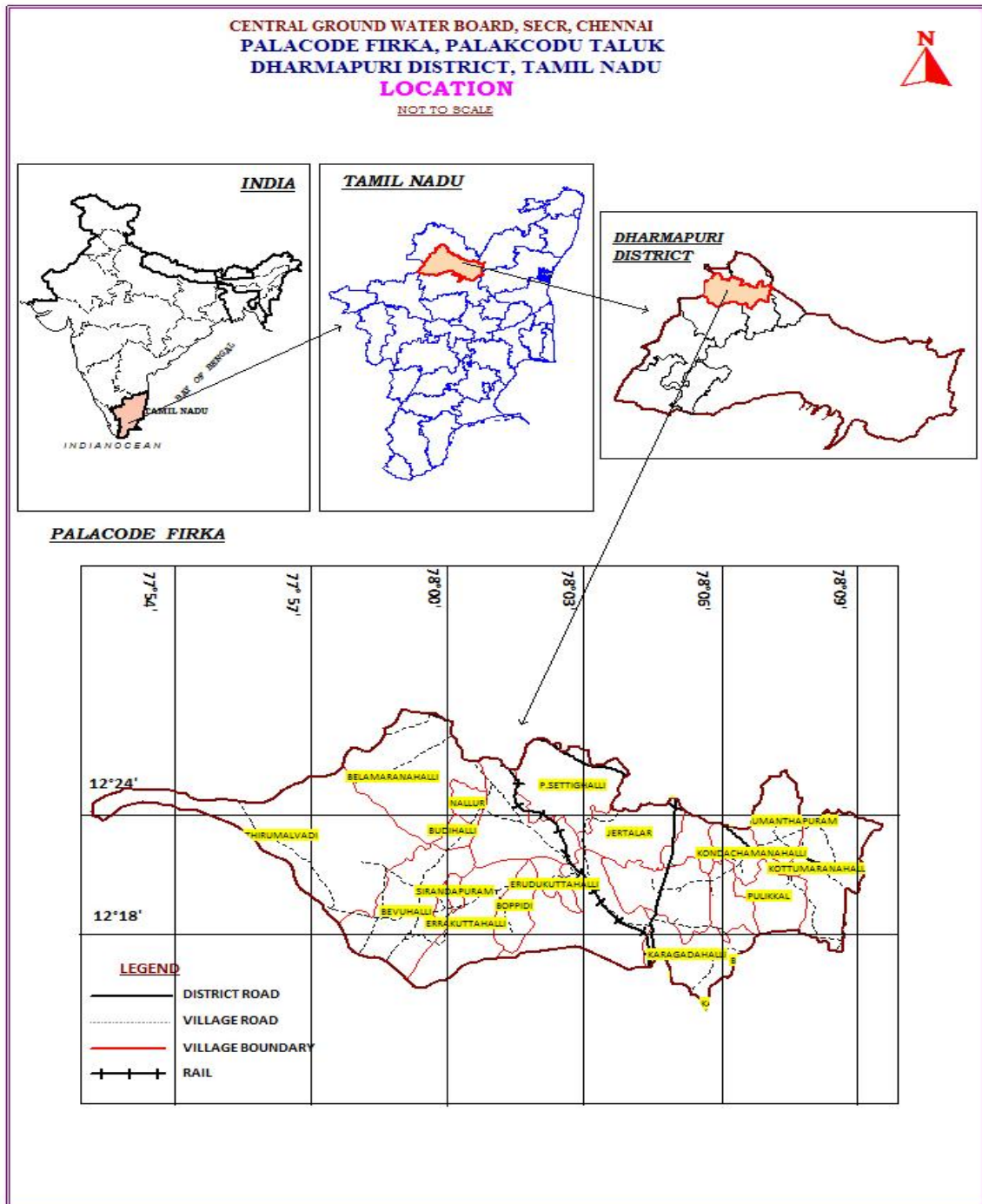
Figure 1. Location map of Palacode firka
