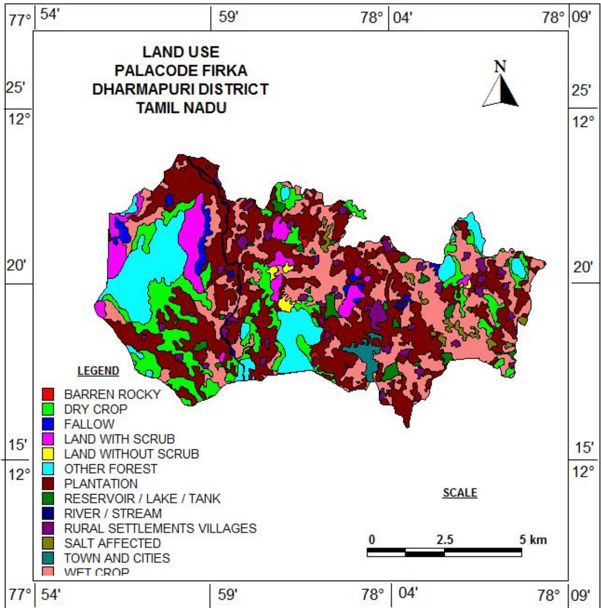
Figure 3. Land use map of Palacode Firka
