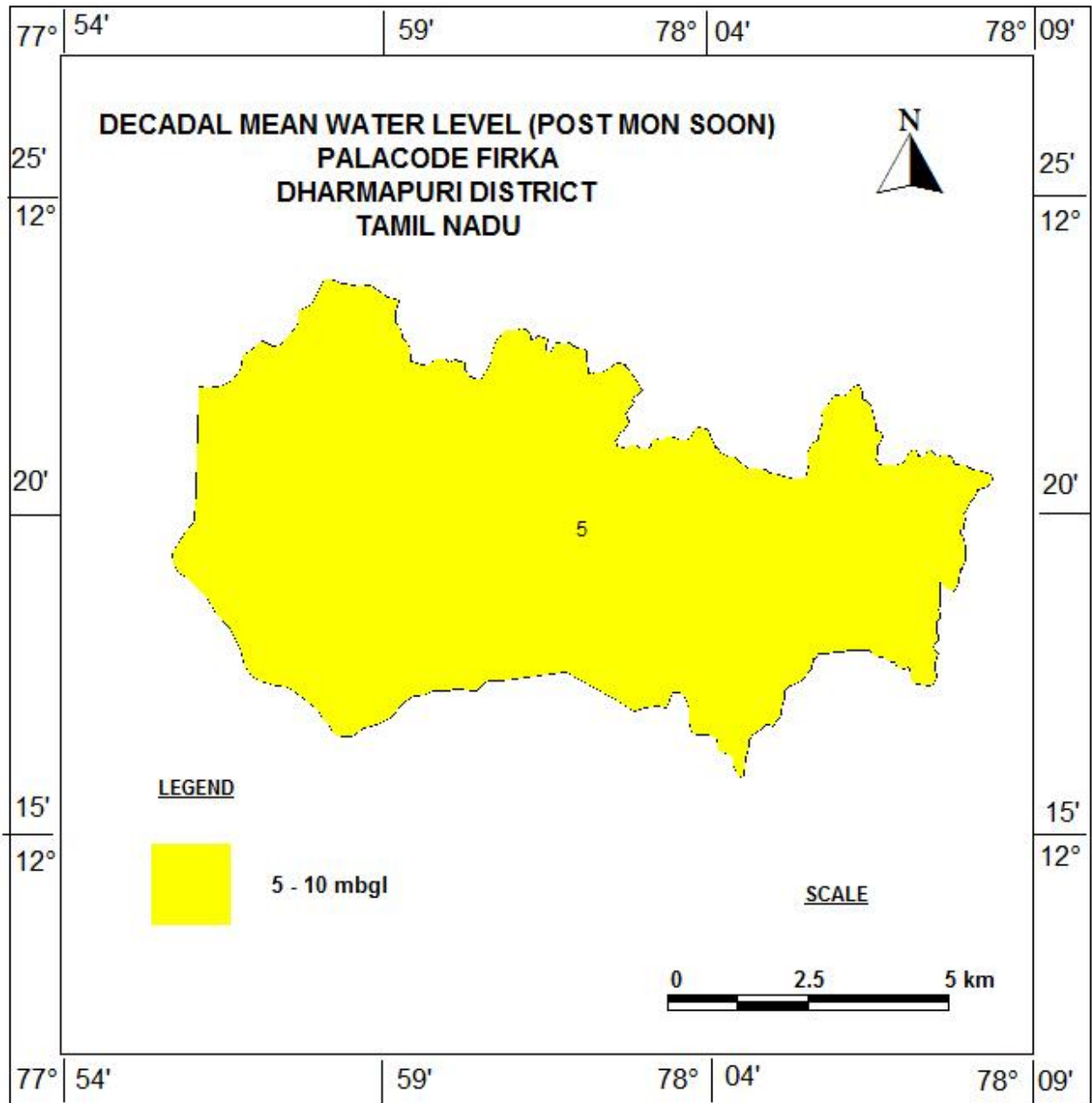
Figure 6 b. Decadal Post-monsoon water level in Placode firka
