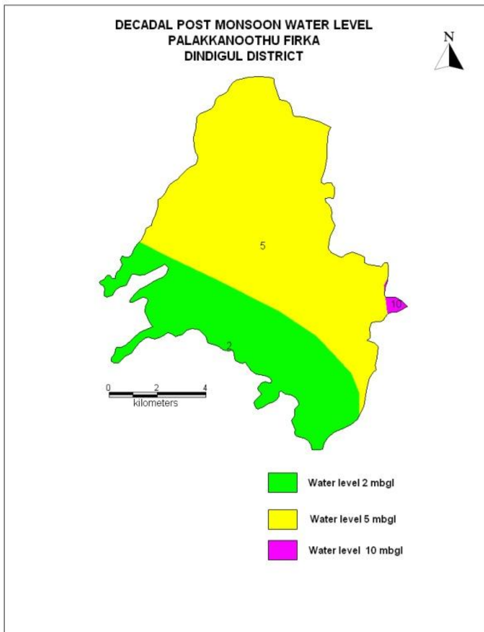
Figure 6b. Post-monsoon water level in Palakkanoothu firka (Decadal)
