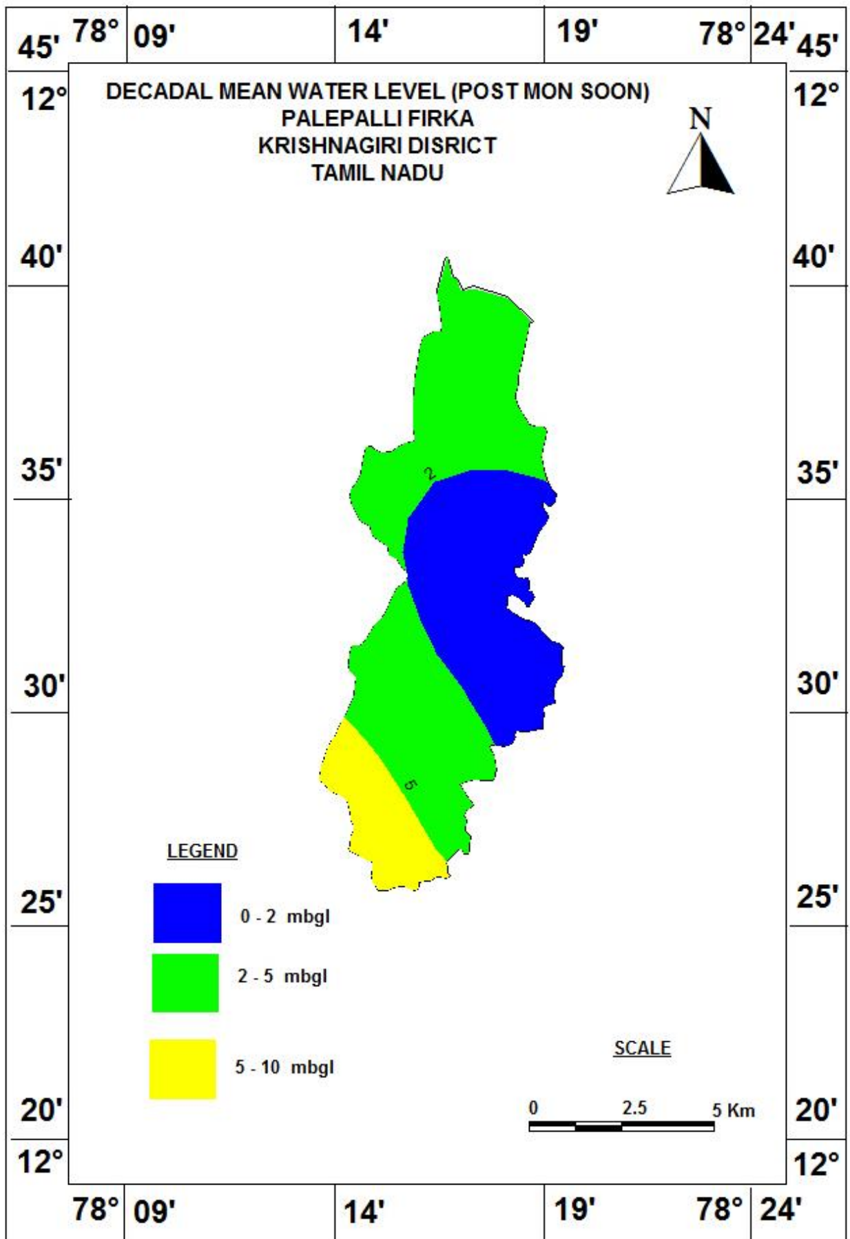
Figure 6 b. Decadal Post-monsoon water level in Palepalli firka
