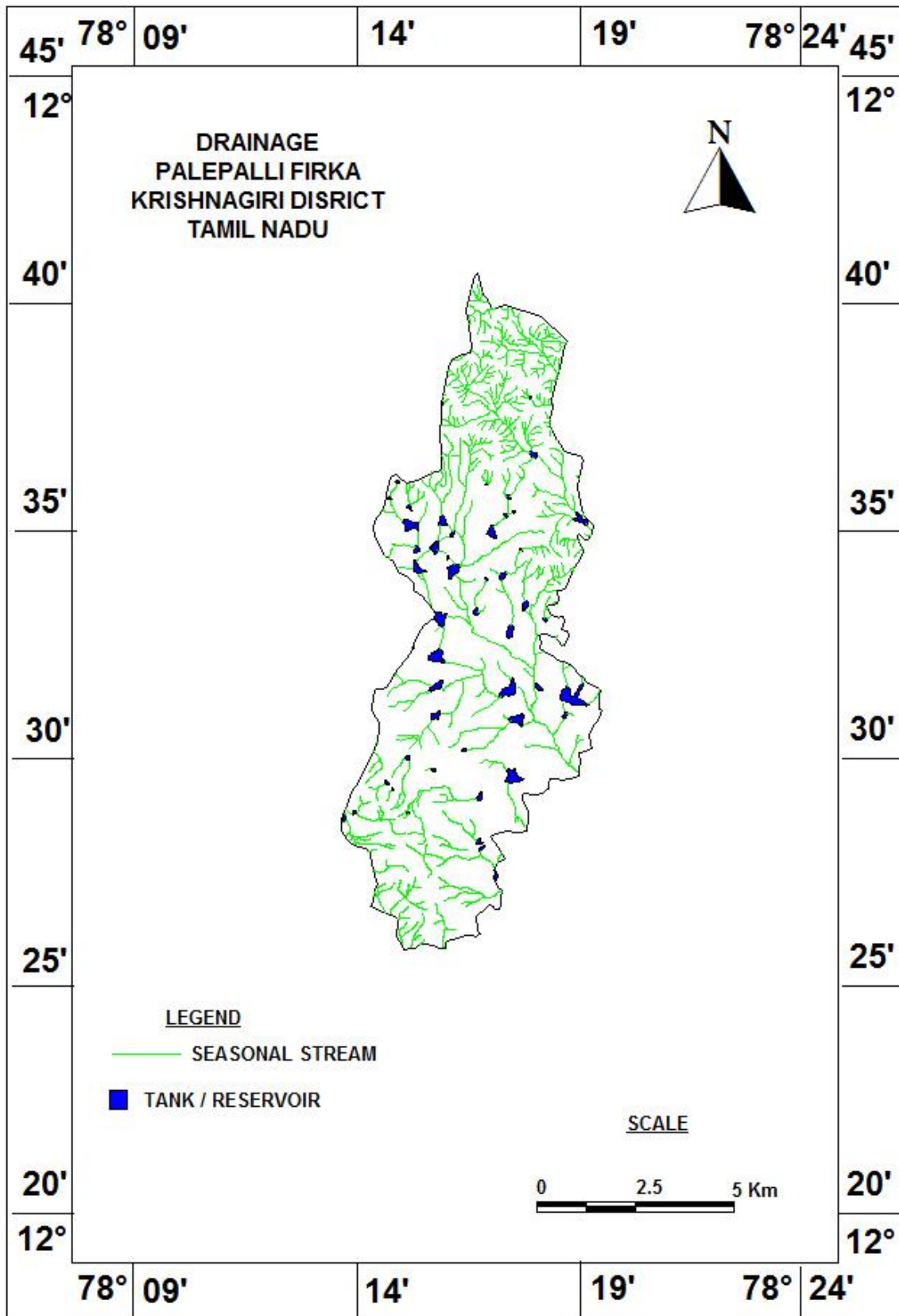
Figure 4. Drainage map of Palepalli firka
