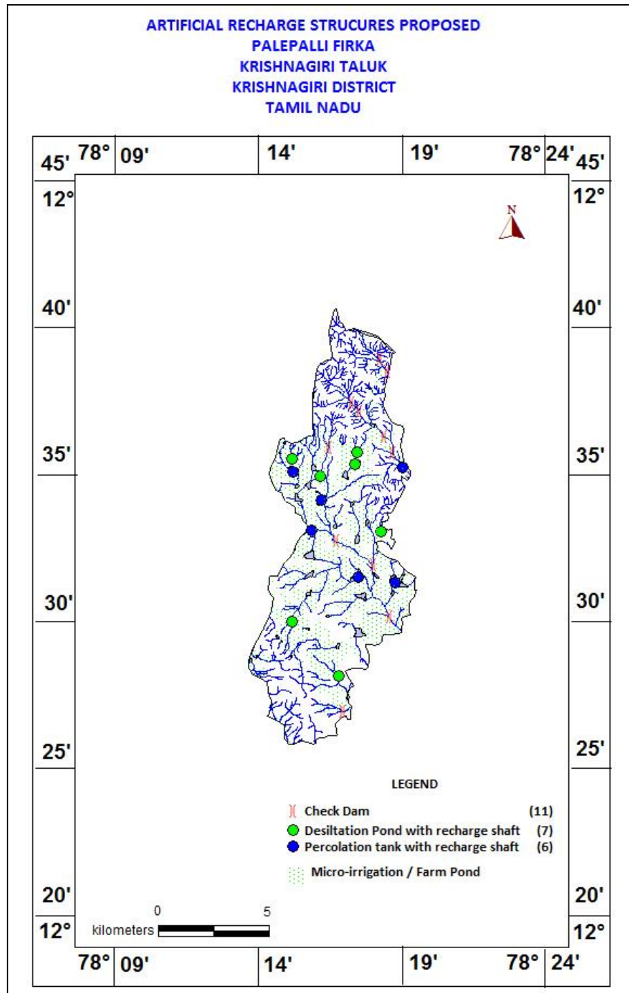
Figure 7. Location map showing the proposed AR Structures
