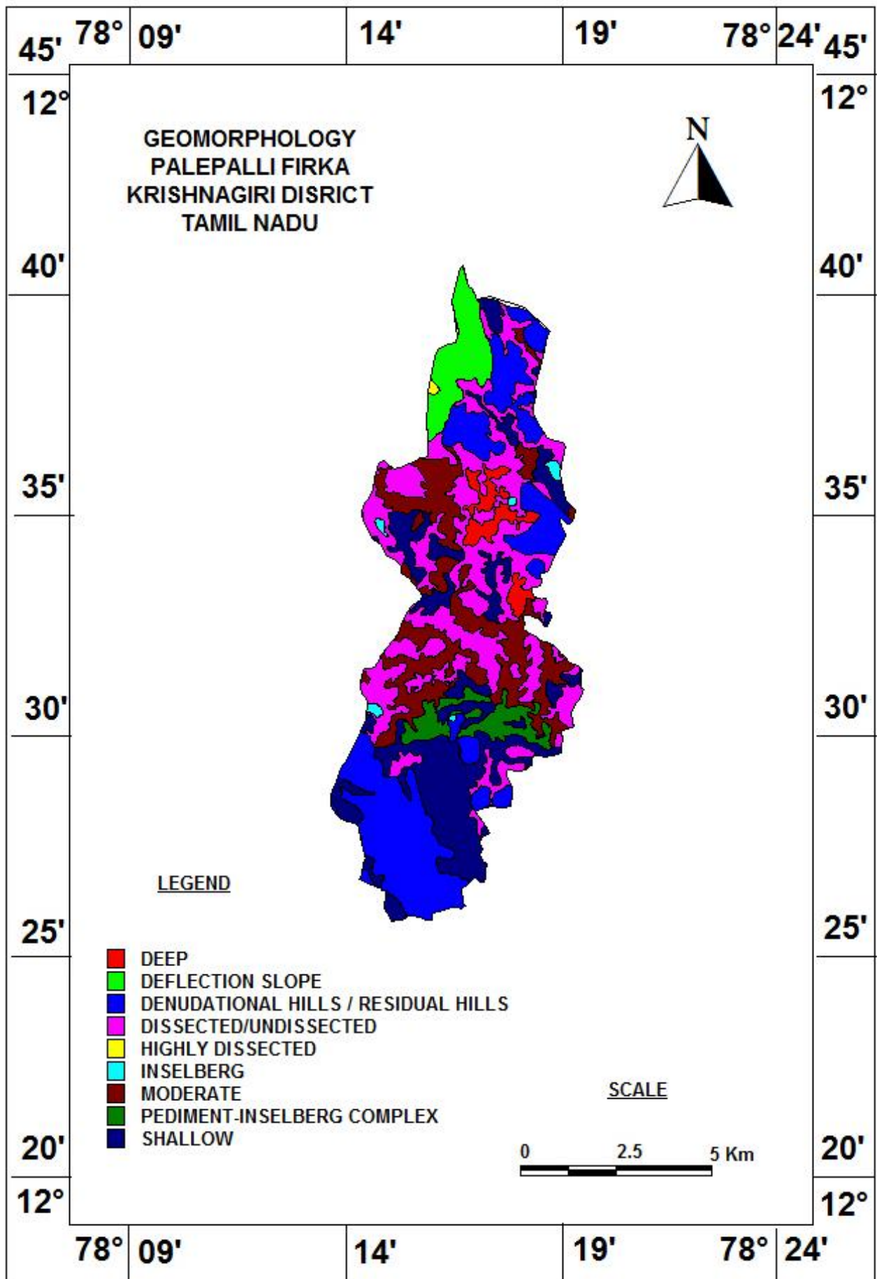
Figure 2. Geomorphology of Palepalli firka
