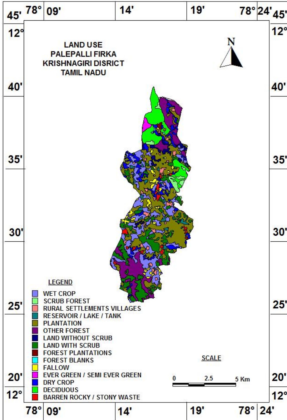
Figure 3. Land use map of Palepalli firka
