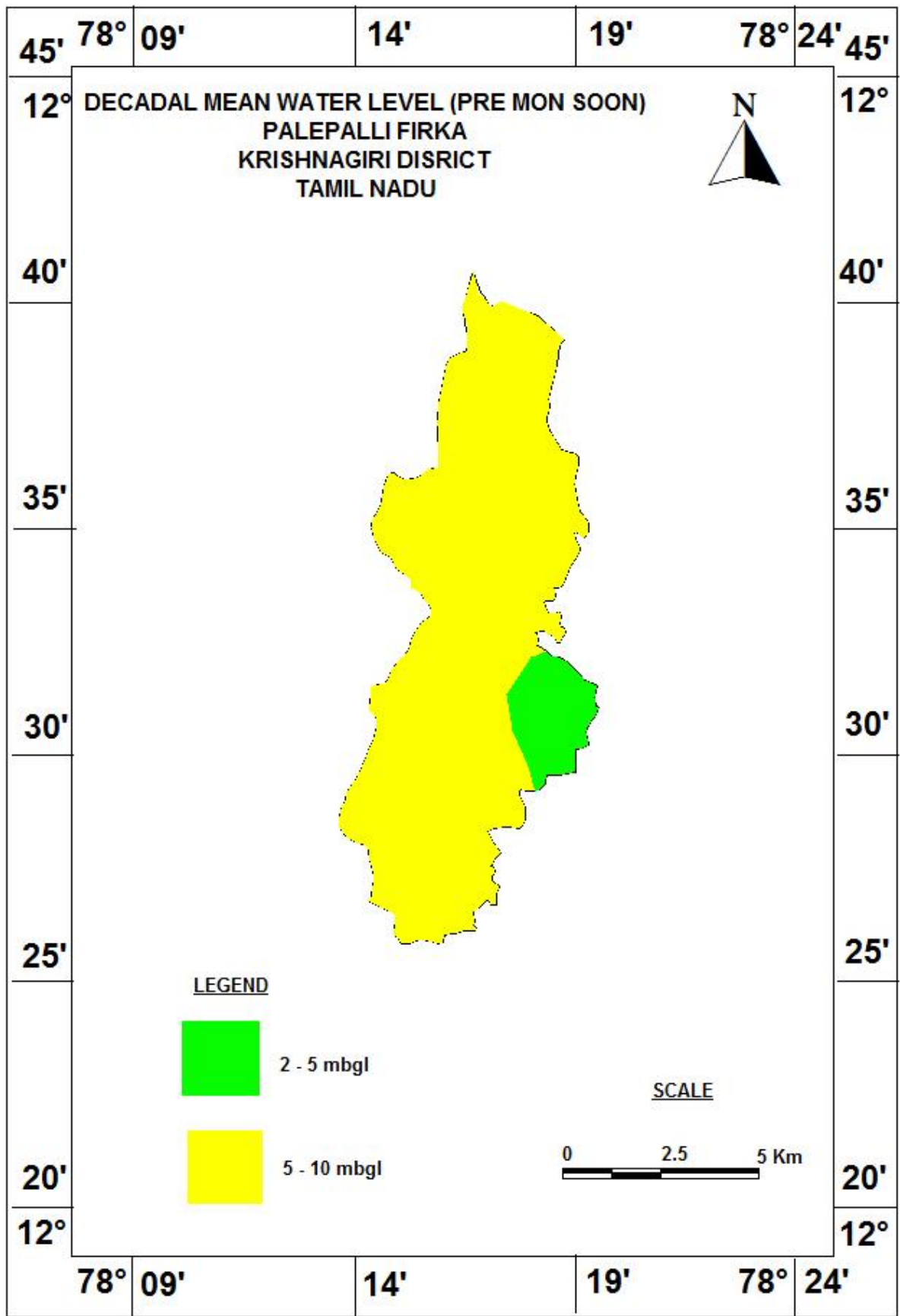
Figure 6a. Decadal Pre -monsoon water level in Palepalli firka
