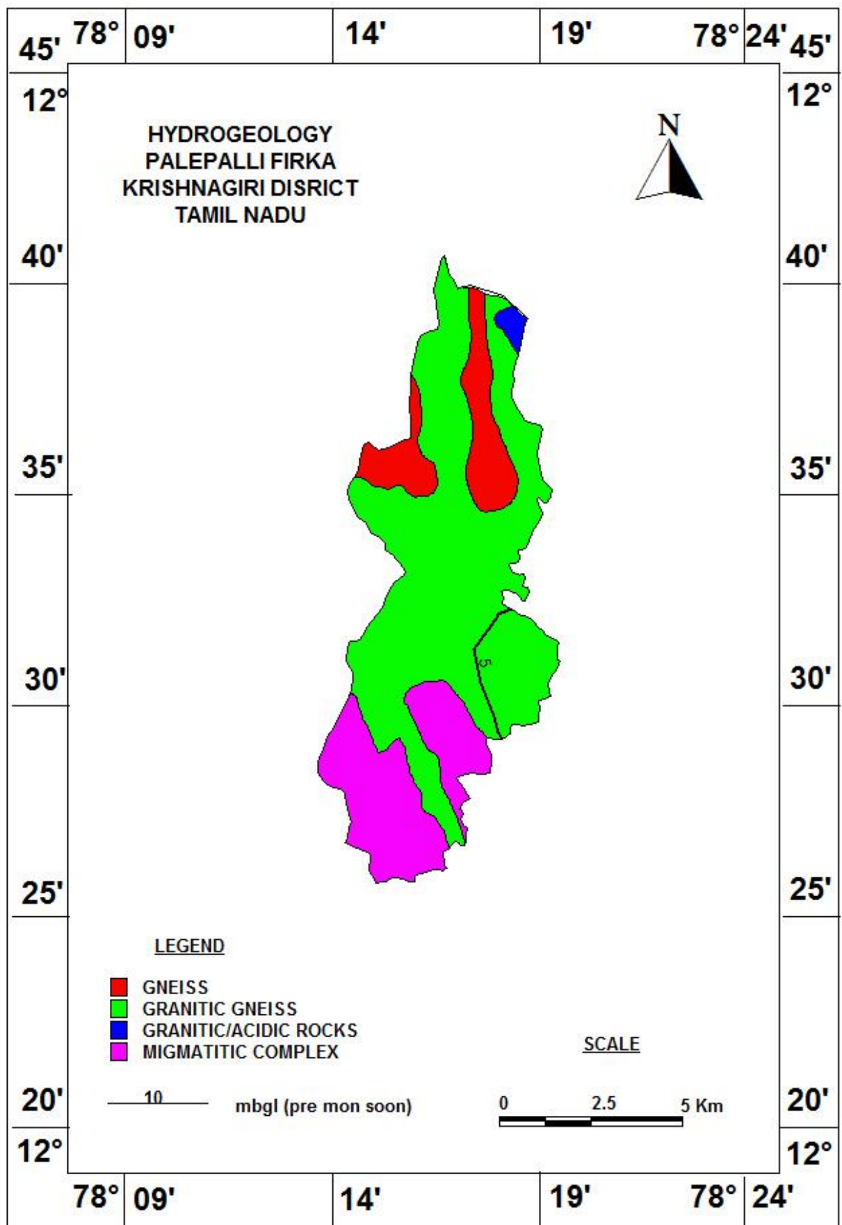
Figure 5. Hydrogeological Map of Palepalli firka
