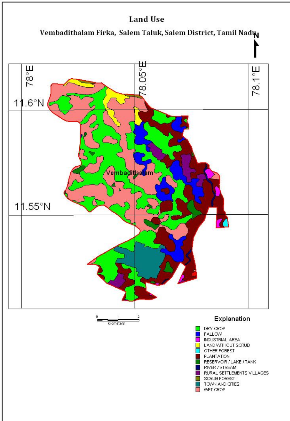
Figure 3. Landuse map of Vembudithalam Firka
