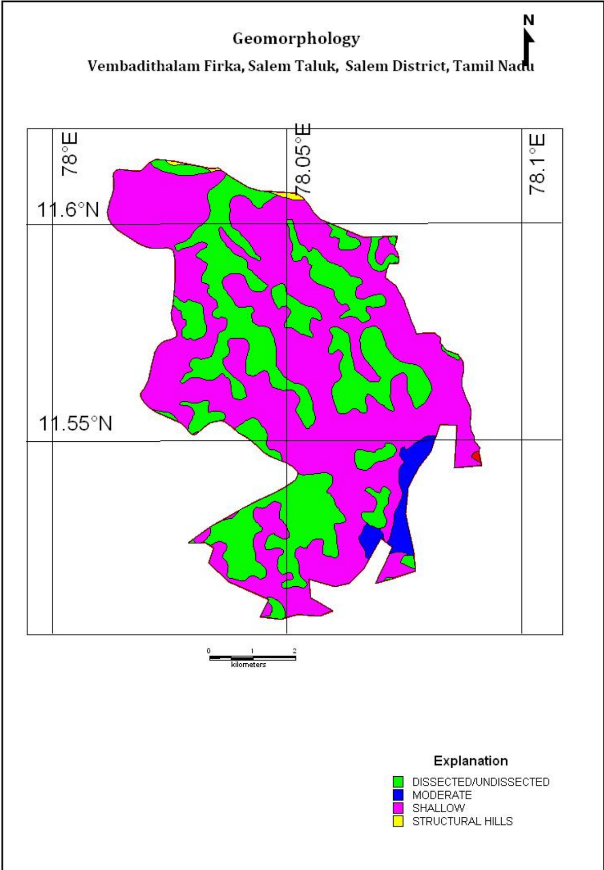
Figure 2. Geomorphology of Vembudithalam Firka
