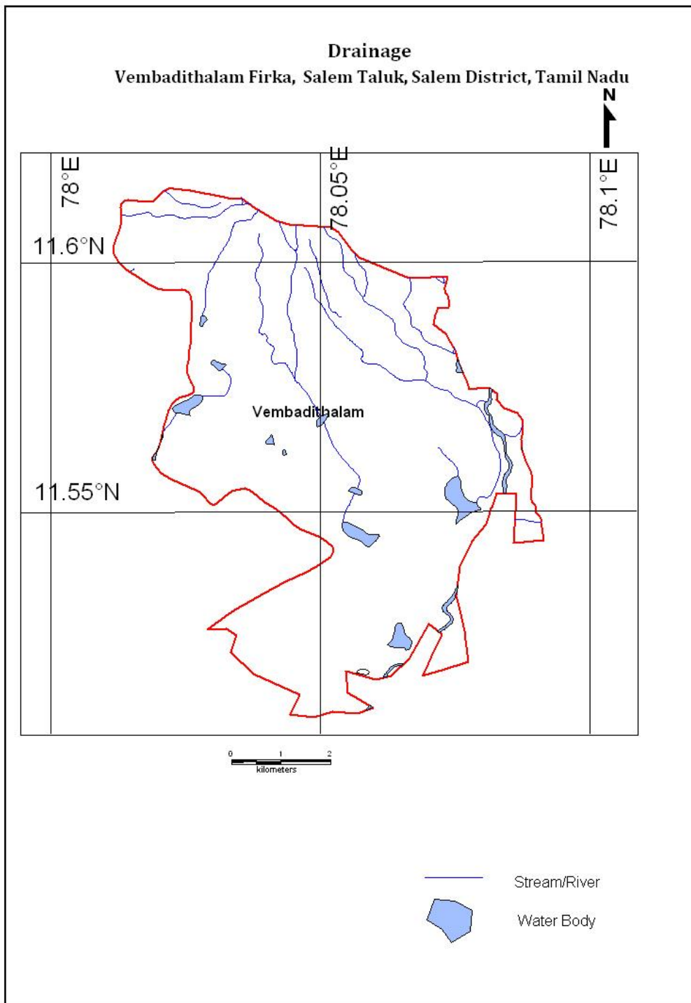
Figure 4. Drainage map of Vembudithalam Firka
