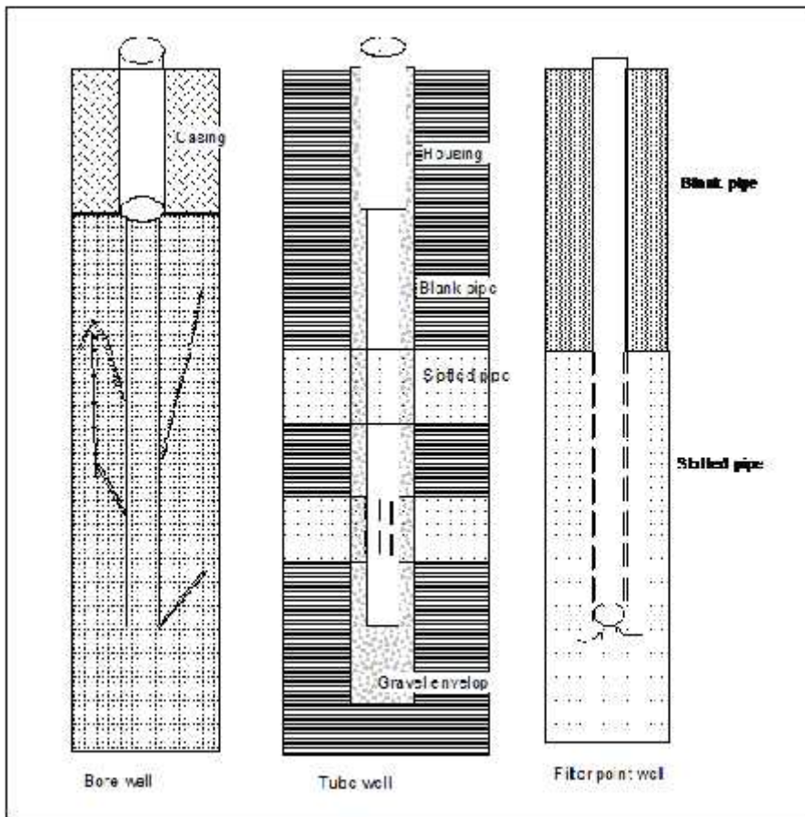
Fig 2 - Well design
