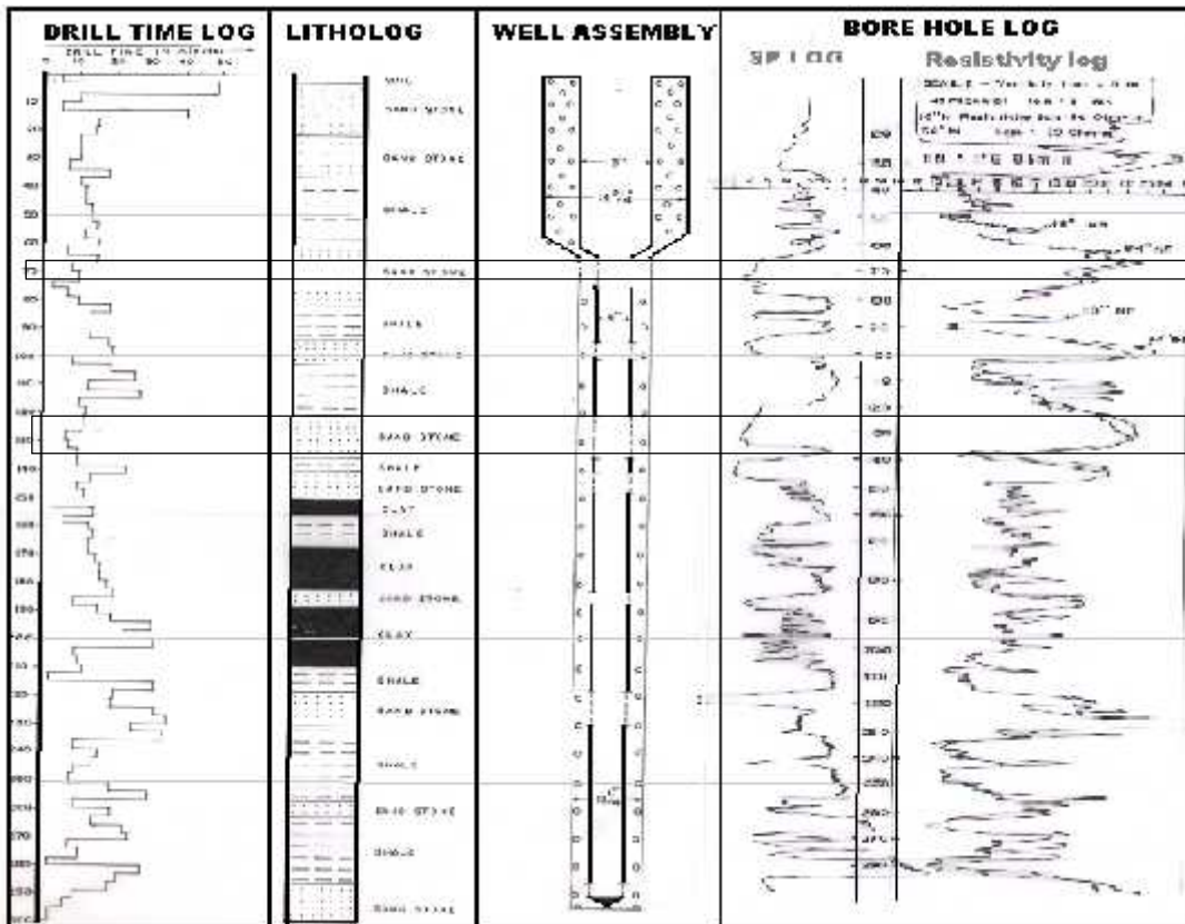
Fig. 3: Design of Kotrimal Bore well and relation with Drill Time Log, Litholog, SP Resistivity Log
