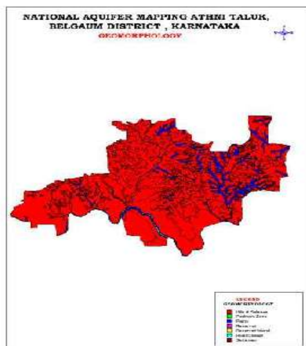
Fig 2: Geomorphology Map
