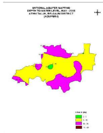
Fig 5: Depth to water level Map-Aq-I (May.2016)
