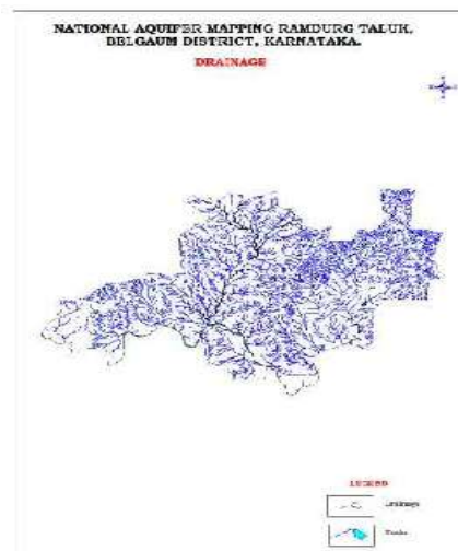
Fig 3: Drainage Map
