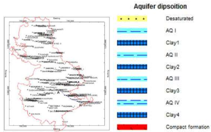
Figure 6A: Section A - A': Uchain-Pichuna-Khandoli-Roopwas-Khansurajpur, Block Weir
