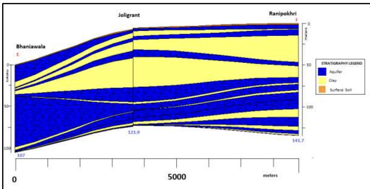
Fig: 3.10 (a): Section Depicting Sub-surface Lithological Variation from Bhaniawala to Ranipokhri 3.10 (b): Section depicting Sub-surface aquifer disposition from Bhaniawala to Ranipokhri
