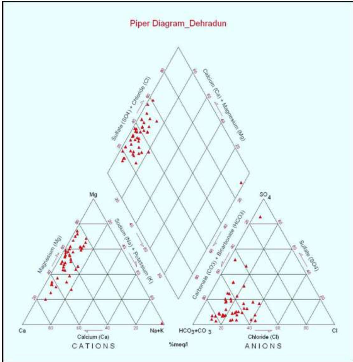
Figure 3.17-- Piper Diagram constructed after analysis of groundwater samples collected from the study area
