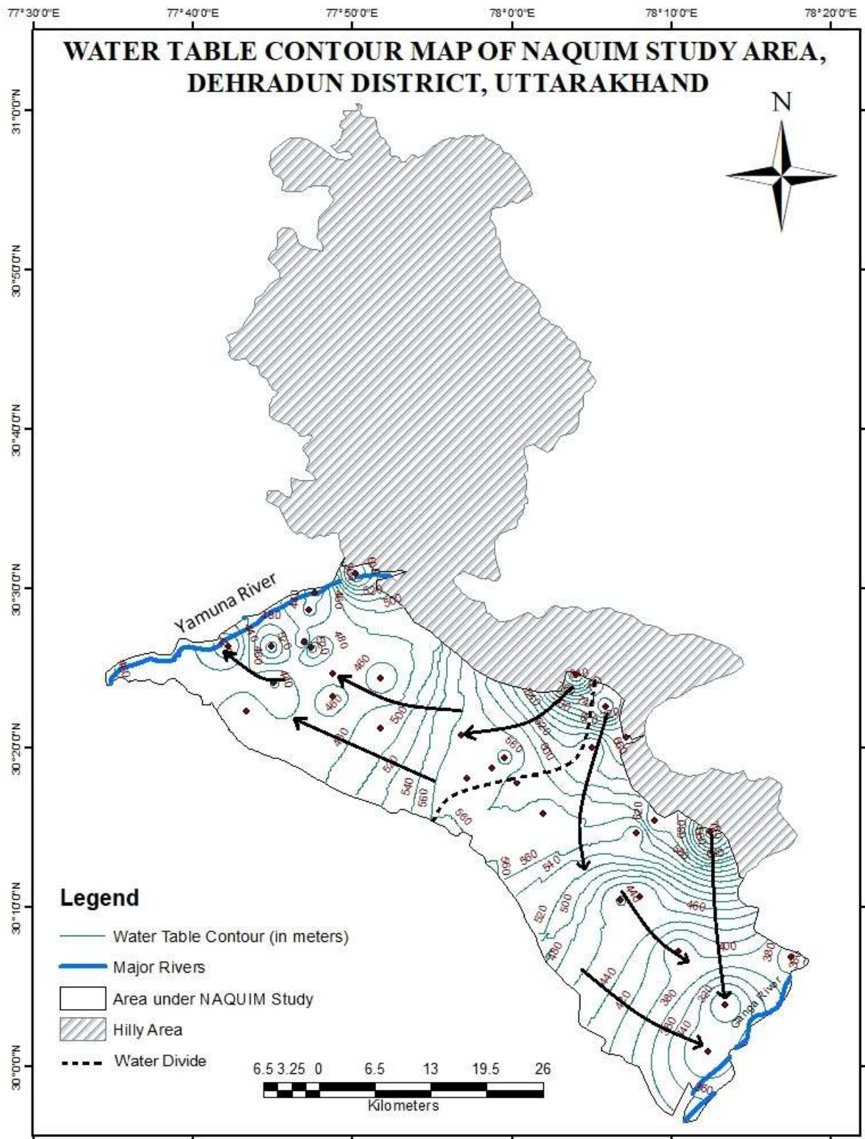
Fig 3.12: Water table Contour map of the Study area showing movement of groundwater
