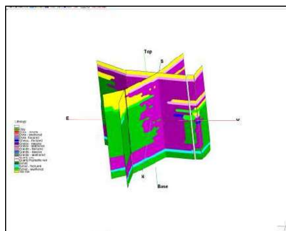
Fig 14. & Fig 15. 3 D Stratigraphy Fence diagrams
