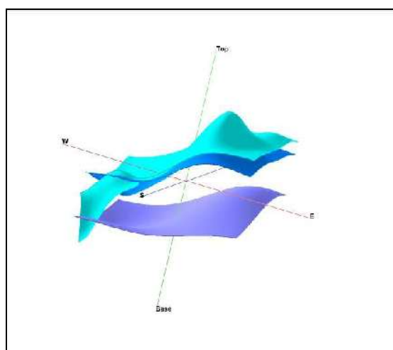
Fig 14. & Fig 15. 3 D Stratigraphy Fence diagrams
