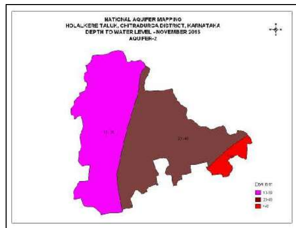
Fig 9. Post- monsoon DTW Aquifer- II
