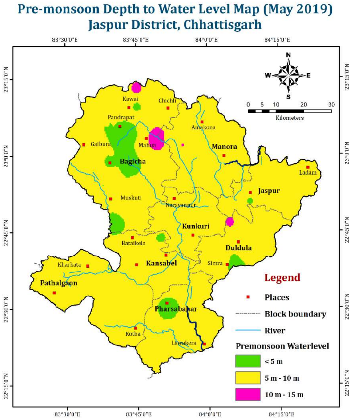
Figure 9 Pre monsoon Water Level Maps of Phreatic Aquifer
