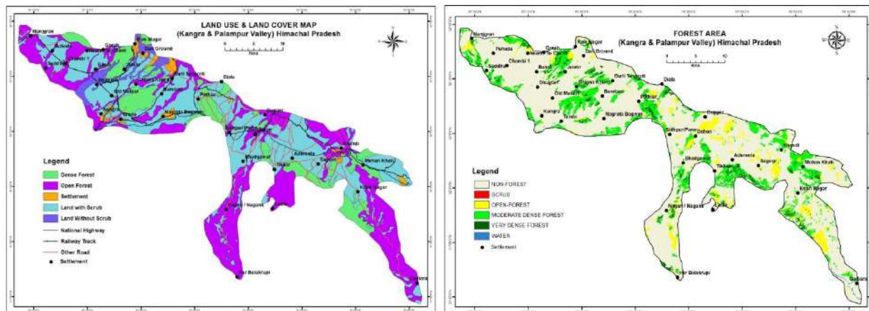
Fig. 1.12 (a) Land Use & Land Cover
