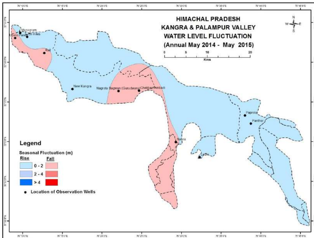
Fig. 2.14 Annual Water Level Fluctuation May 2014 & May 2015, Kangra & Palampur Valley, Himachal Pradesh
