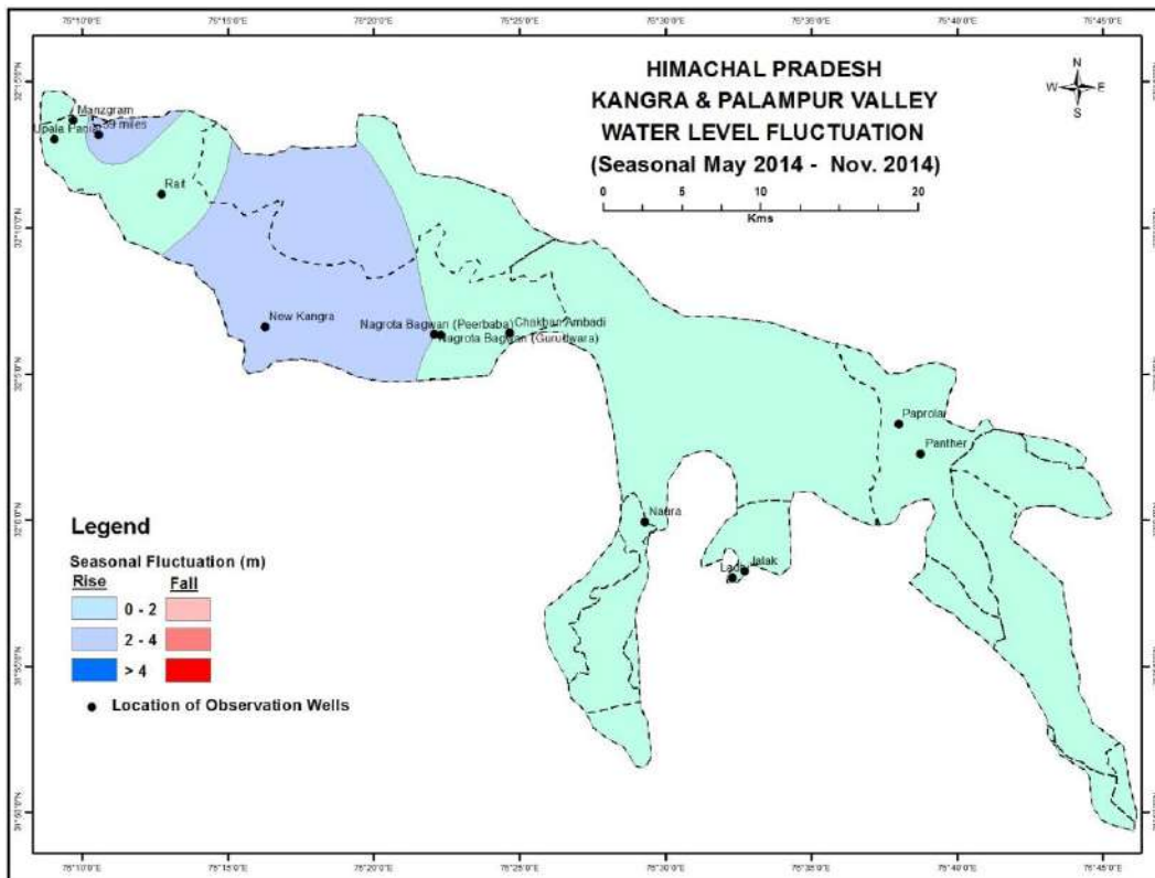
Fig. 2.2 Seasonal Water Level Fluctuation – May 2014 & November 2014, Kangra & Palampur Valley, Himachal Pradesh
