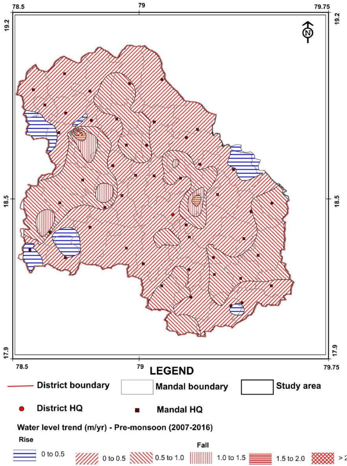
Fig. 2.8: Long-term water level trends (Pre-monsoon-2007-16).
