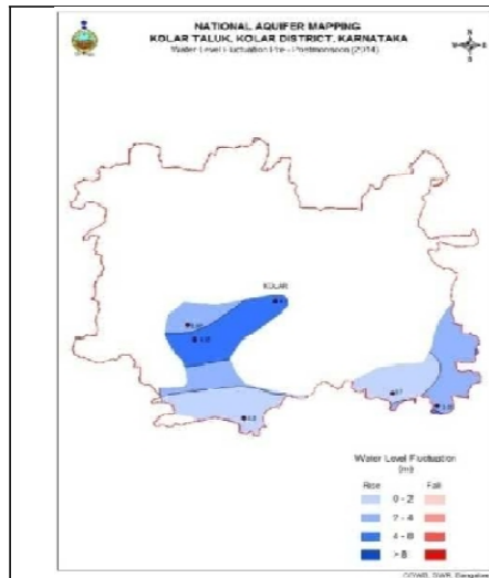
Fig. 10: Water level fluctuation (Aq – I)
