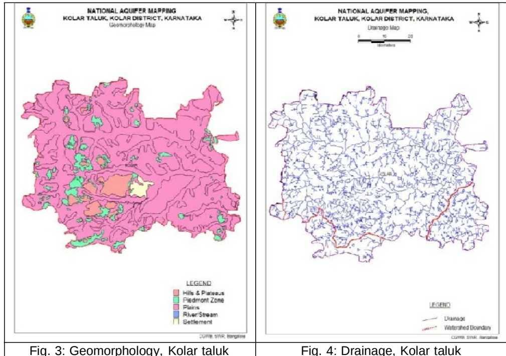
Fig. 3: Geomorphology, Kolar taluk
