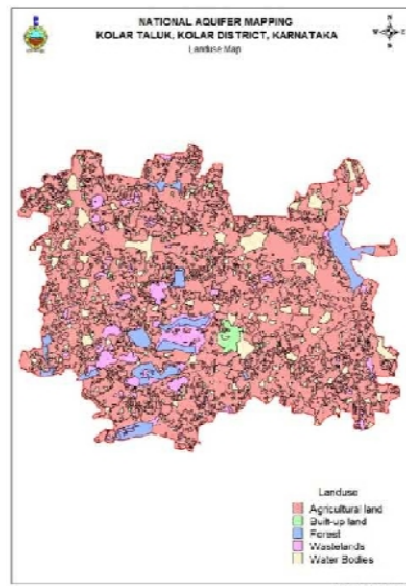
Fig. 2: Land use, Kolar taluk
