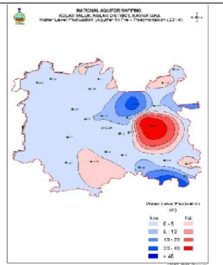
Fig. 11: Water level fluctuation (Aq – II)
