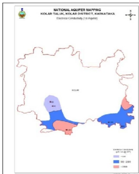
Fig 24: Electrical Conductivity (Aq-I)
