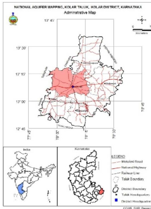
Fig 1: Location map of Kolar taluk, Kolar district
