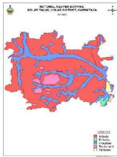
Fig. 5: Soil map, Kolar taluk
