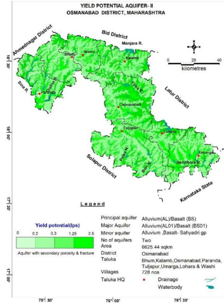
Figure 2. 7: Yield Potential, Aquifer-II
