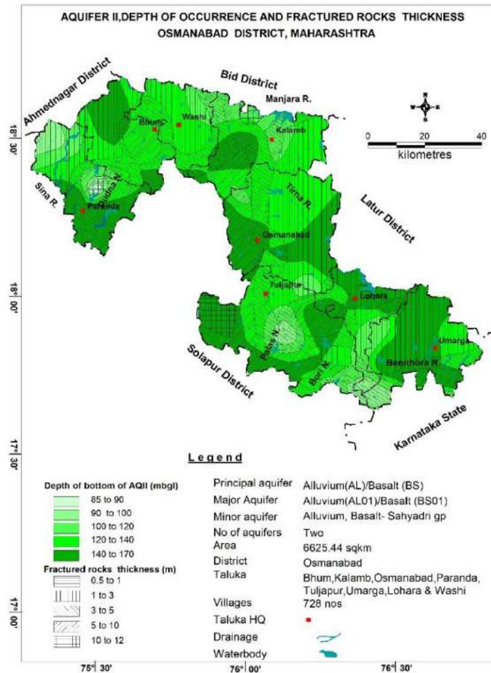
Figure 2. 6: Depth of Occurrence and Fractured rock thickness-Aquifer-II
