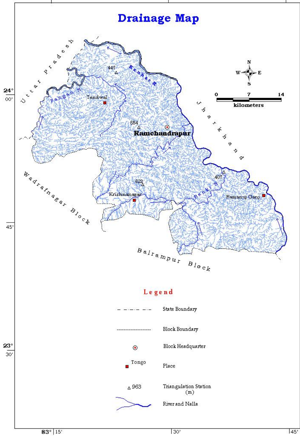
Figure 3 Drainage Map of Ramchandrapur Block
