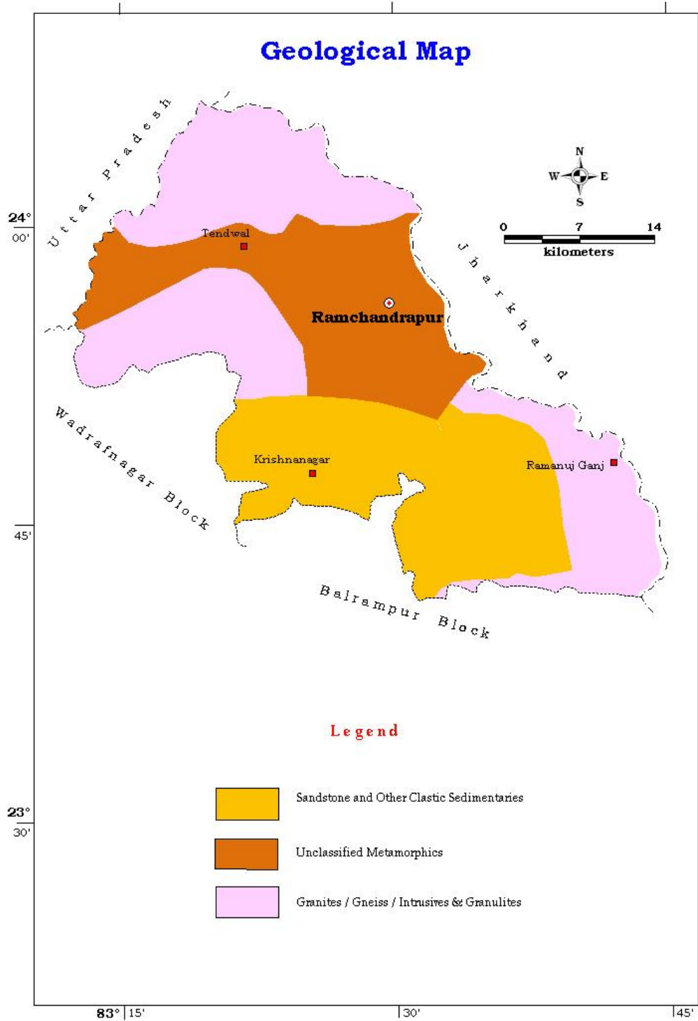
figure 11: Aquifer map of Ramchandrapur block
