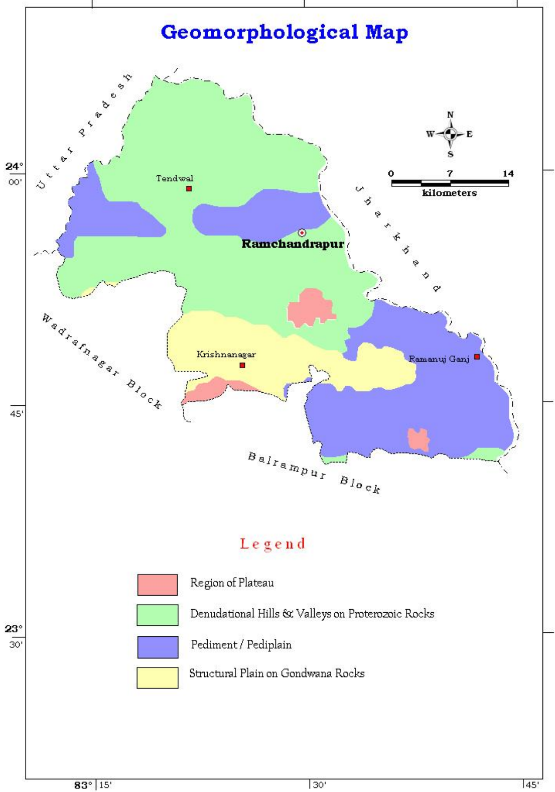
Figure 2 Geomorphology Map of Ramchandrapur Block
