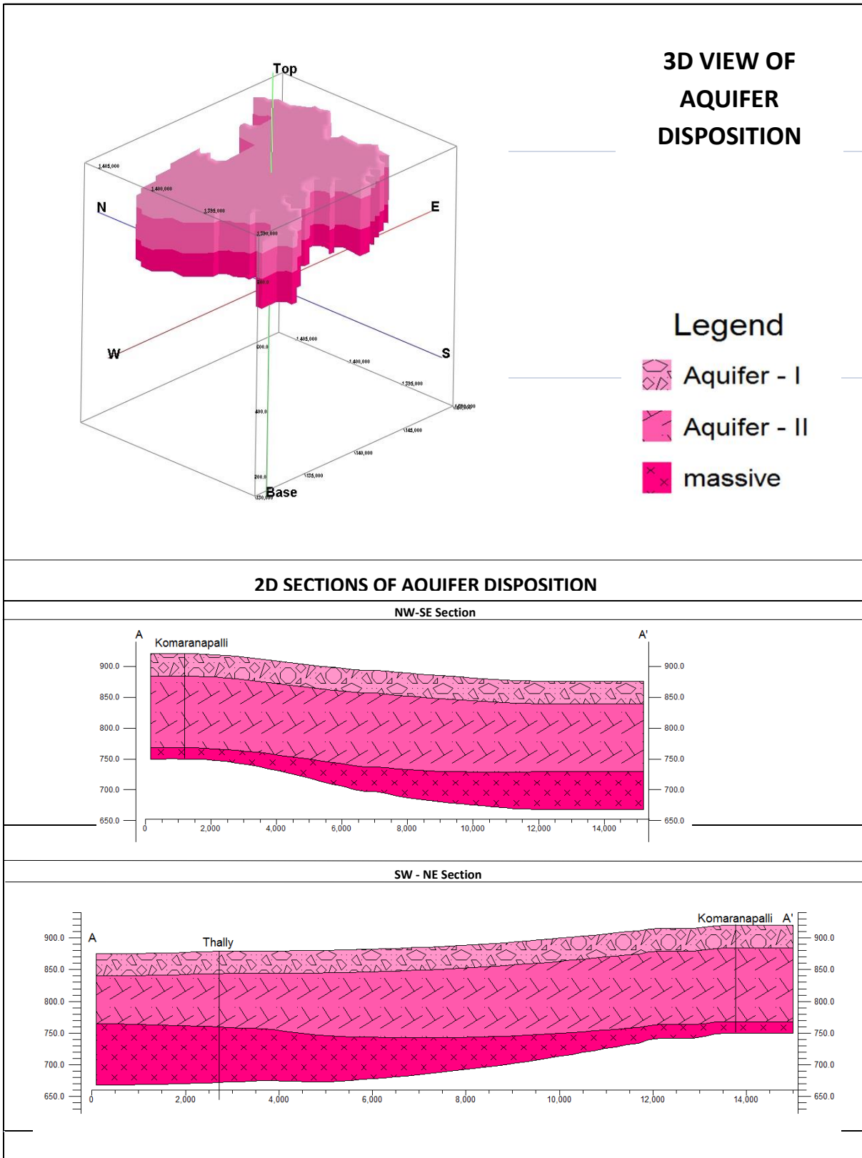
Fig:2 3D and 2D View of Aquifer Disposition, Thally Firka, Krishnagiri District
