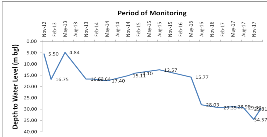
Fig. 6.10 Well Hydrograph (GMMW) at Maneri (UK-HP-7A)
