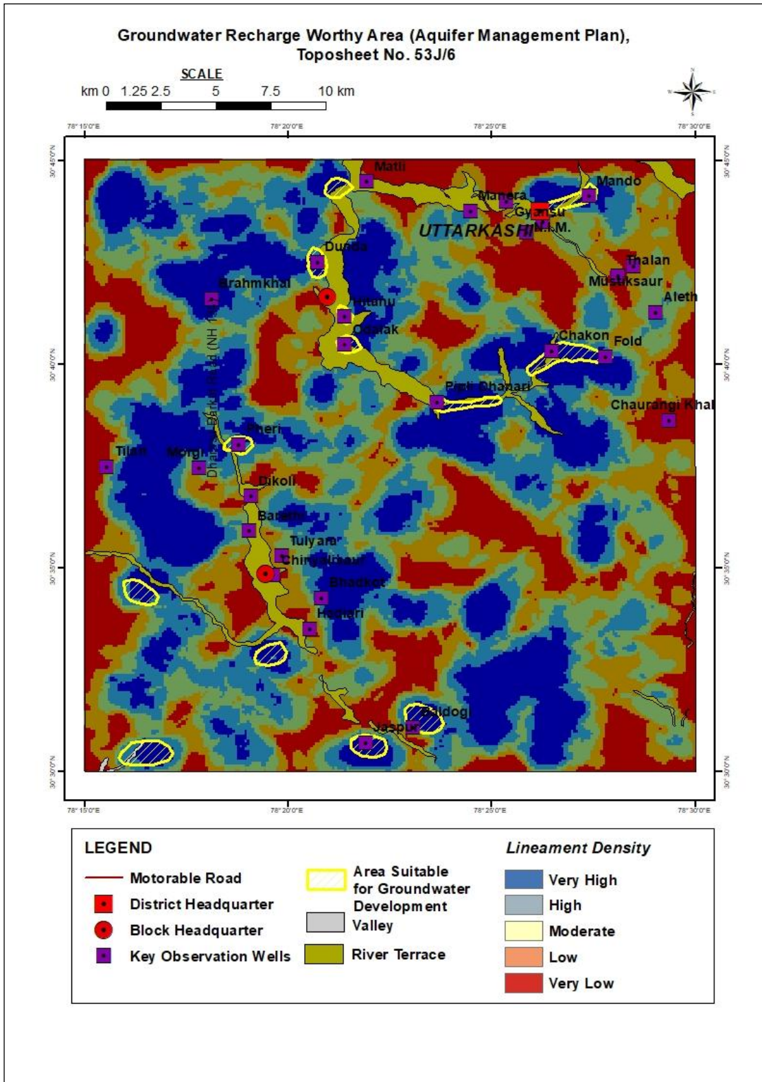
Fig. 7.1 Aquifer Management Plan showing areas suitable for groundwater Development, Toposheet No. 53J/6, Uttarkashi District
