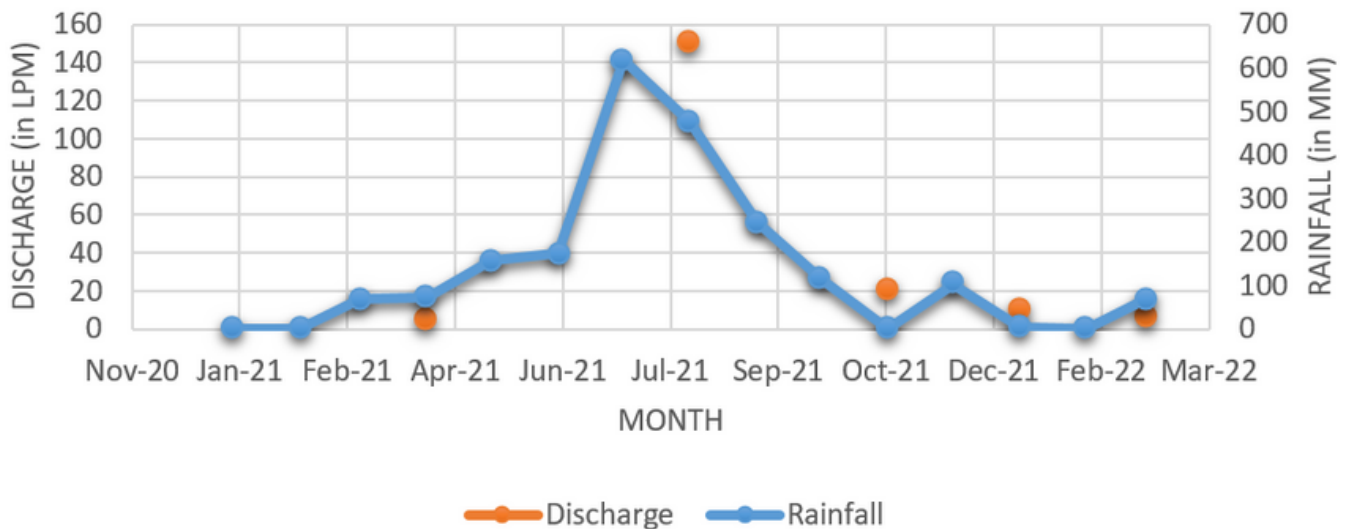
Discharge (lpm) of Vangmun spring vs Rainfall (mm) Kanchanpur station for the year 2021
